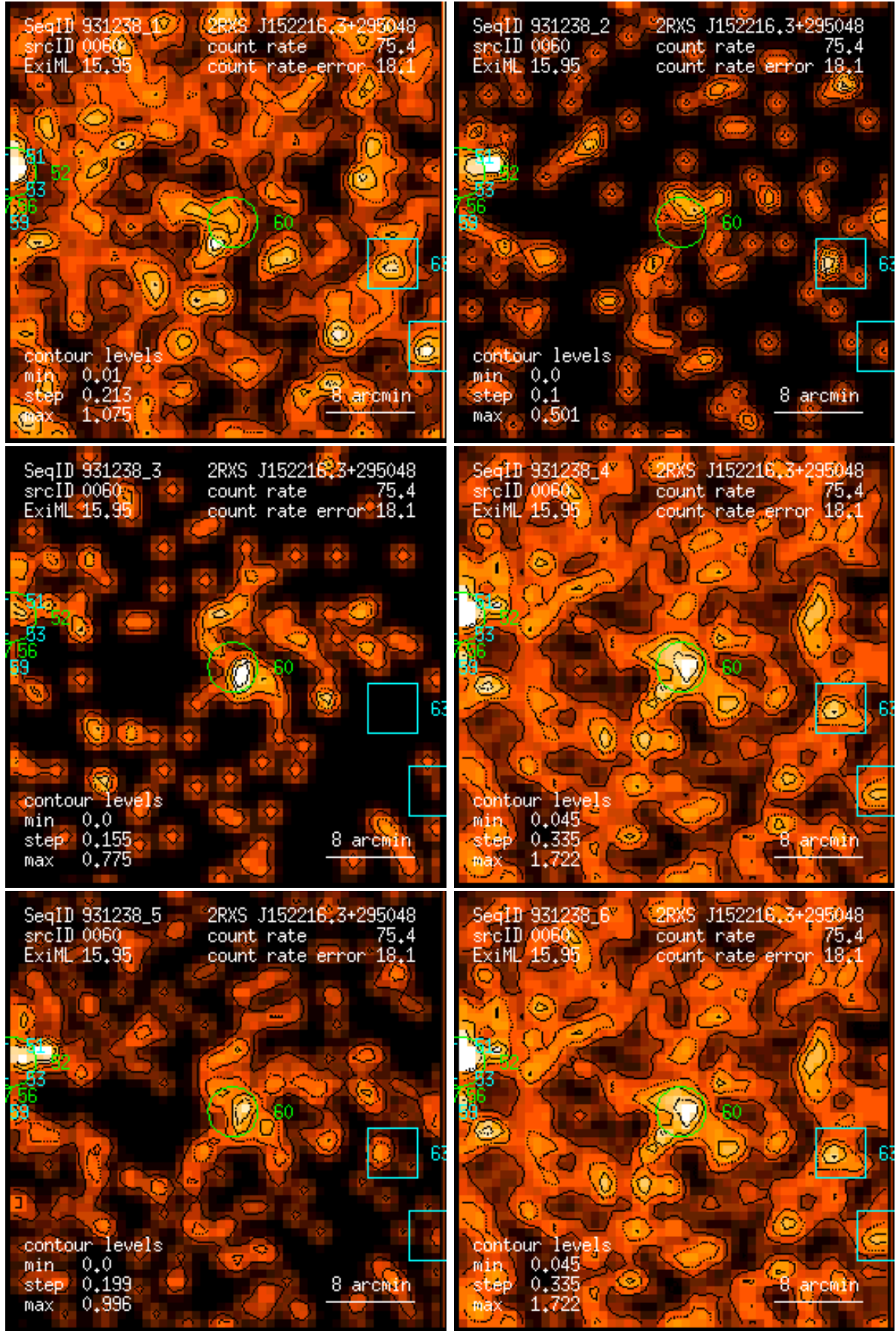
Figure 60: RASS 931238: detection 0060: band rate images, Gaussian filter: (1) PSPC channels 11 – 41, (2) 52 – 90, (3) 91 – 201, (4) 11 – 235, (5) 52 – 201, (6) 11 – 201. Broad band rates in counts/ks. Band rate contour levels in counts/ks/arcmin 2 .
