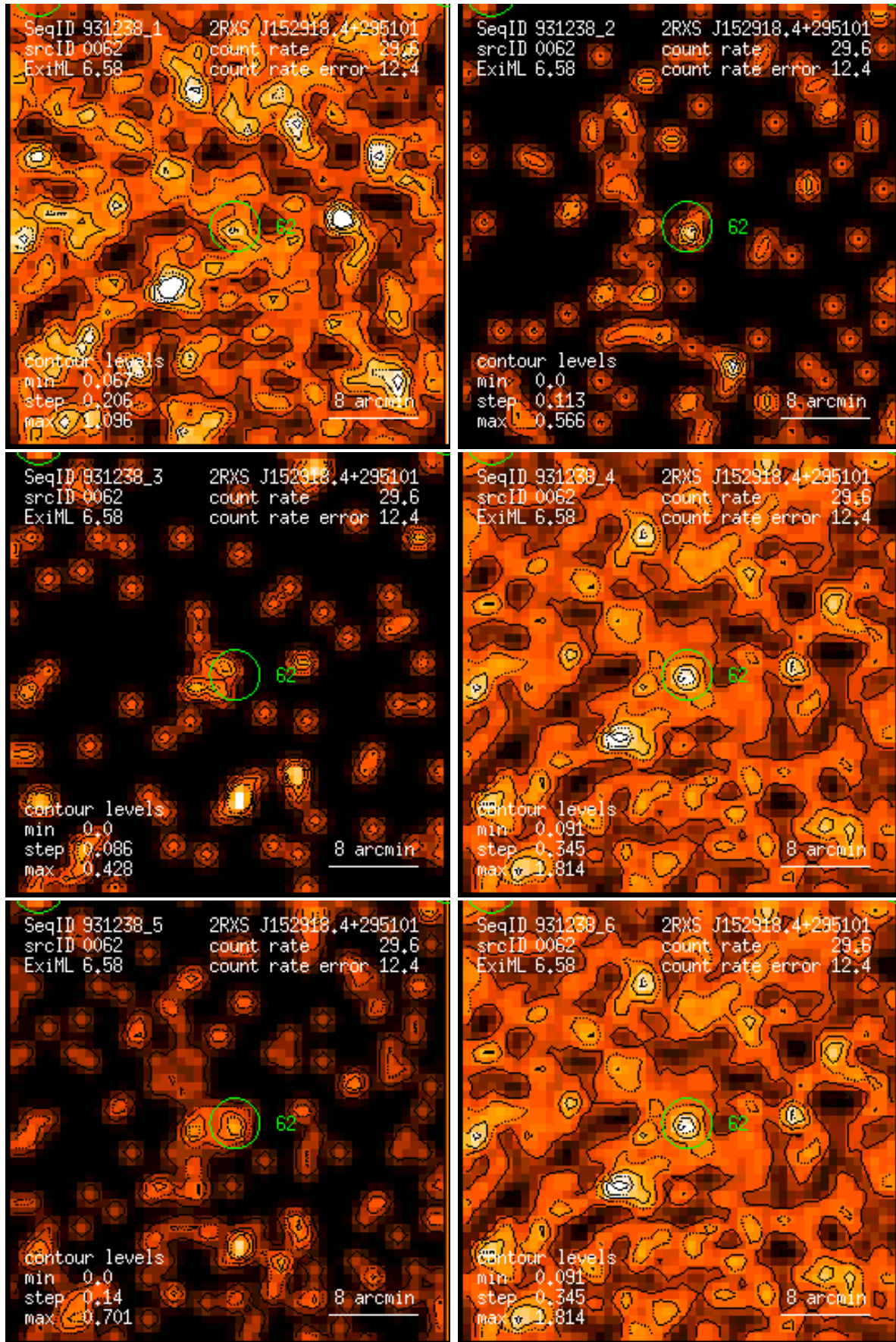
Figure 62: RASS 931238: detection 0062: band rate images, Gaussian filter: (1) PSPC channels 11 – 41, (2) 52 – 90, (3) 91 – 201, (4) 11 – 235, (5) 52 – 201, (6) 11 – 201. Broad band rates in counts/ks. Band rate contour levels in counts/ks/arcmin 2 .
