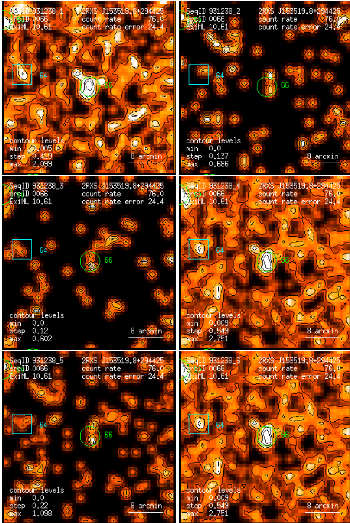
Figure 66: RASS 931238: detection 0066: band rate images, Gaussian filter: (1) PSPC channels 11 – 41, (2) 52 – 90, (3) 91 – 201, (4) 11 – 235, (5) 52 – 201, (6) 11 – 201. Broad band rates in counts/ks. Band rate contour levels in counts/ks/arcmin 2 .
