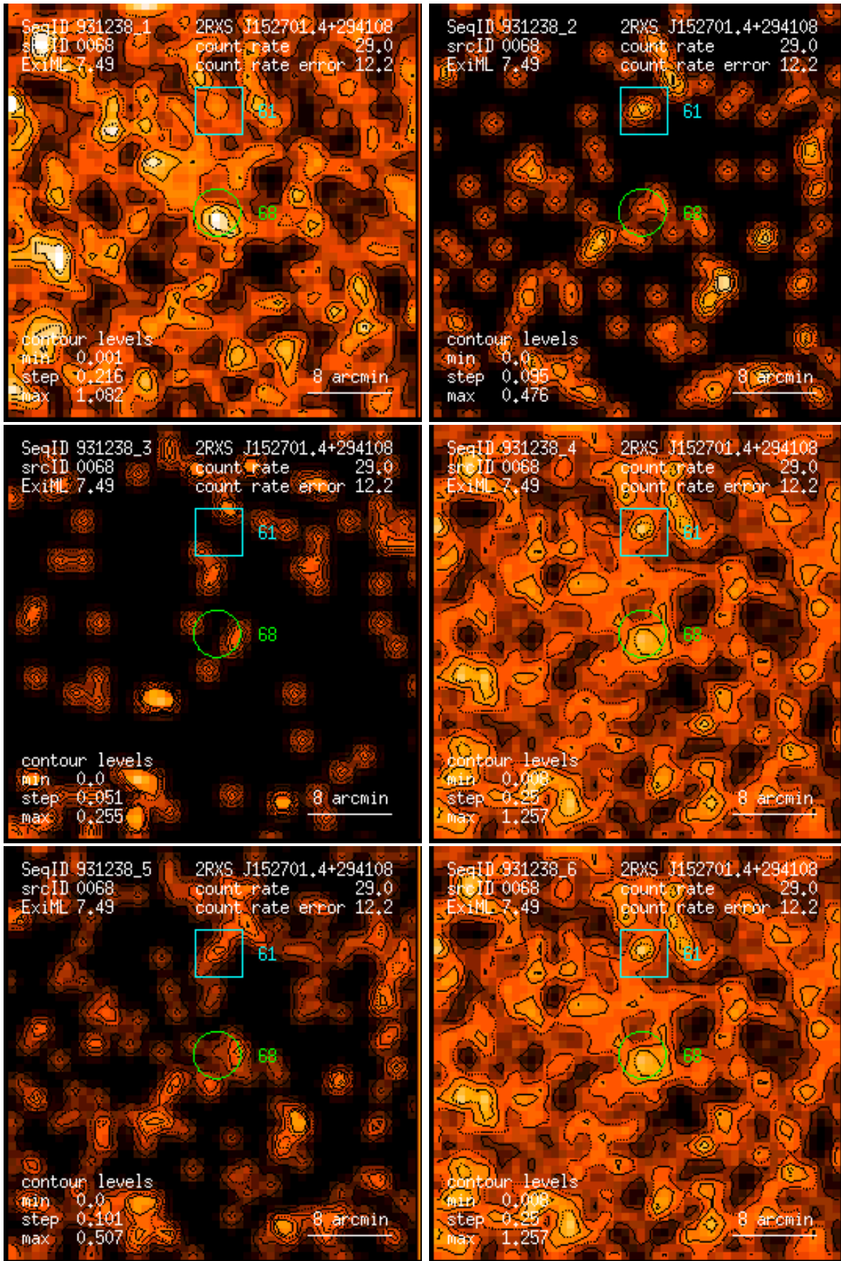
Figure 68: RASS 931238: detection 0068: band rate images, Gaussian filter: (1) PSPC channels 11 – 41, (2) 52 – 90, (3) 91 – 201, (4) 11 – 235, (5) 52 – 201, (6) 11 – 201. Broad band rates in counts/ks. Band rate contour levels in counts/ks/arcmin 2 .
