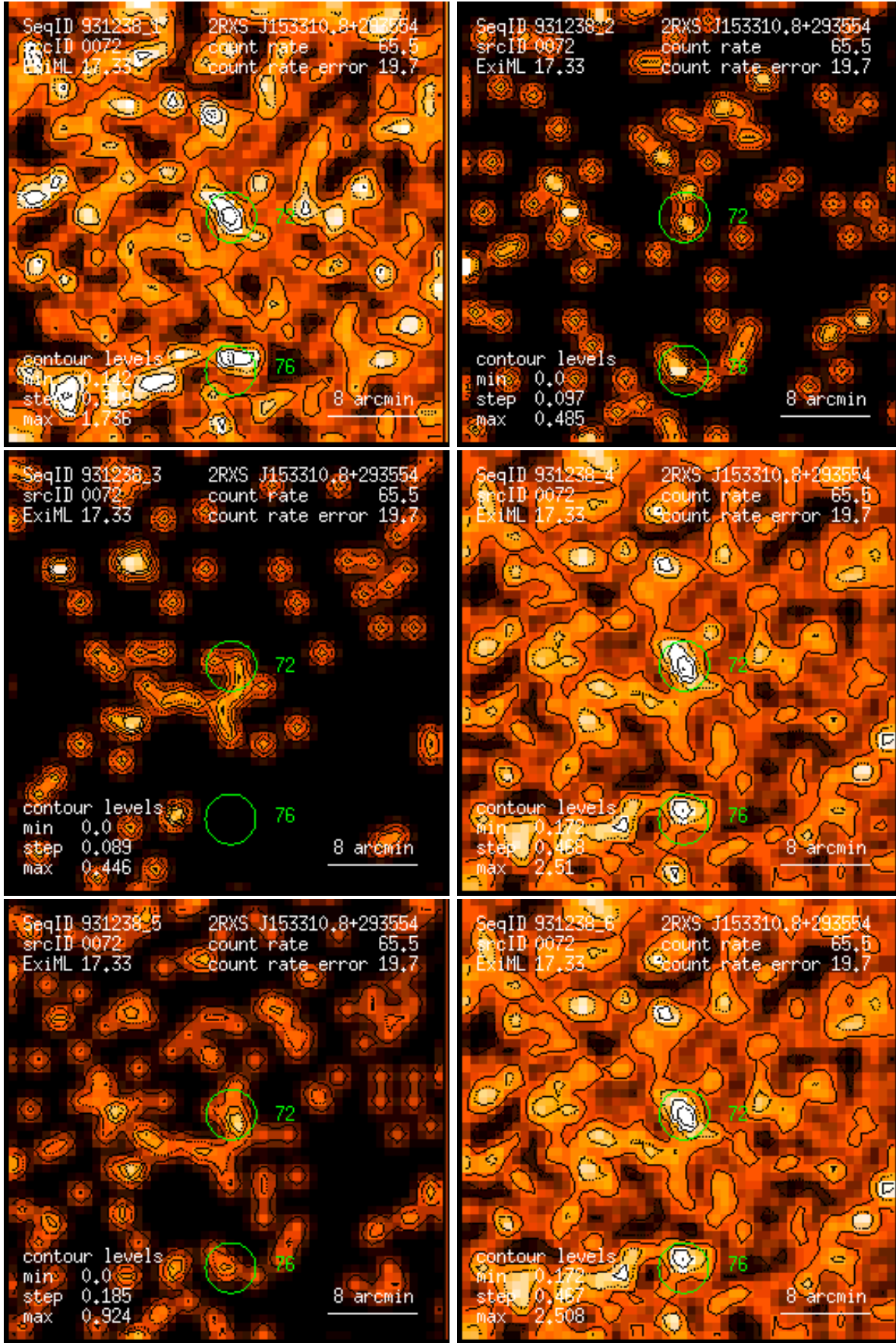
Figure 72: RASS 931238: detection 0072: band rate images, Gaussian filter: (1) PSPC channels 11 – 41, (2) 52 – 90, (3) 91 – 201, (4) 11 – 235, (5) 52 – 201, (6) 11 – 201. Broad band rates in counts/ks. Band rate contour levels in counts/ks/arcmin 2 .
