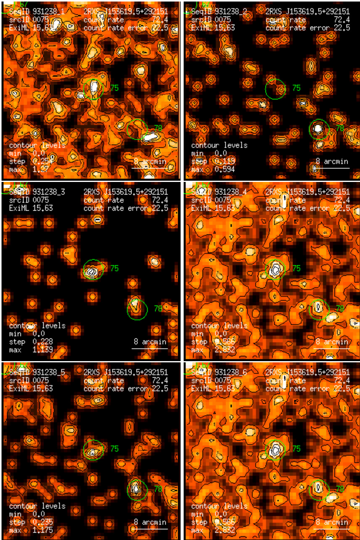
Figure 75: RASS 931238: detection 0075: band rate images, Gaussian filter: (1) PSPC channels 11 – 41, (2) 52 – 90, (3) 91 – 201, (4) 11 – 235, (5) 52 – 201, (6) 11 – 201. Broad band rates in counts/ks. Band rate contour levels in counts/ks/arcmin 2 .
