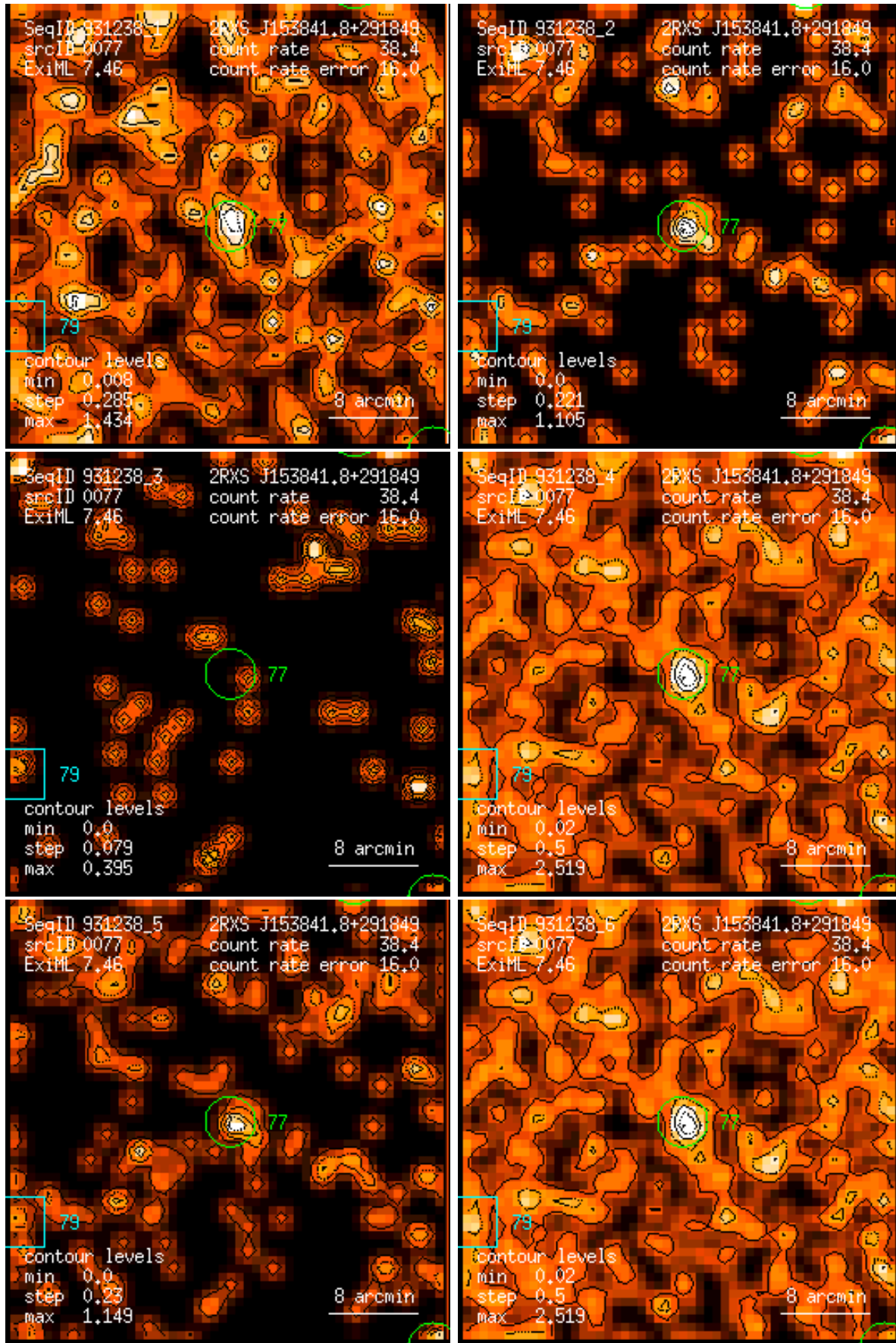
Figure 77: RASS 931238: detection 0077: band rate images, Gaussian filter: (1) PSPC channels 11 – 41, (2) 52 – 90, (3) 91 – 201, (4) 11 – 235, (5) 52 – 201, (6) 11 – 201. Broad band rates in counts/ks. Band rate contour levels in counts/ks/arcmin 2 .
