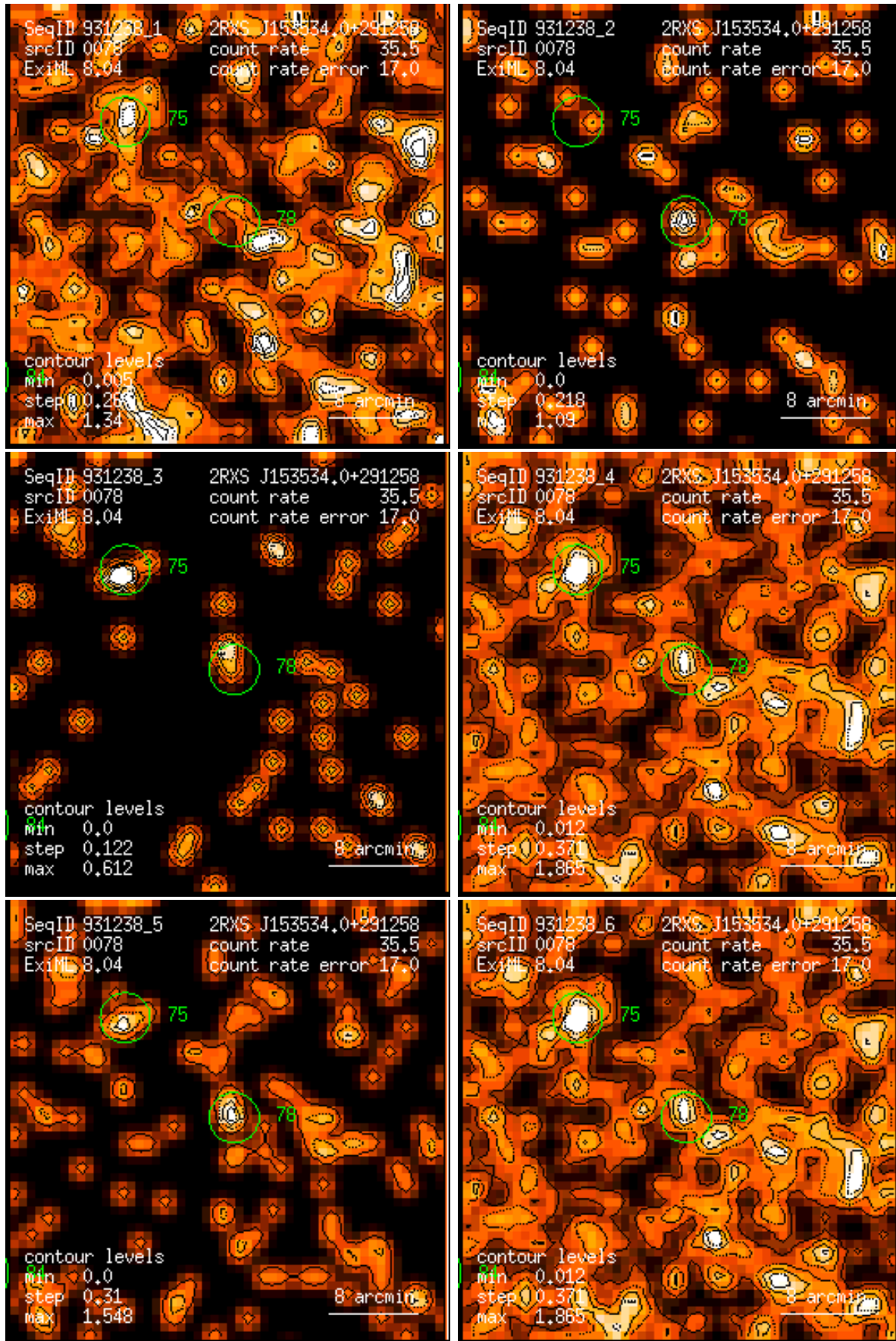
Figure 78: RASS 931238: detection 0078: band rate images, Gaussian filter: (1) PSPC channels 11 – 41, (2) 52 – 90, (3) 91 – 201, (4) 11 – 235, (5) 52 – 201, (6) 11 – 201. Broad band rates in counts/ks. Band rate contour levels in counts/ks/arcmin 2 .
