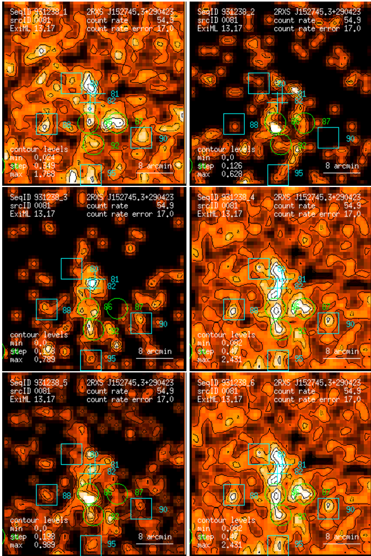
Figure 81: RASS 931238: detection 0081: band rate images, Gaussian filter: (1) PSPC channels 11 – 41, (2) 52 – 90, (3) 91 – 201, (4) 11 – 235, (5) 52 – 201, (6) 11 – 201. Broad band rates in counts/ks. Band rate contour levels in counts/ks/arcmin 2 .
