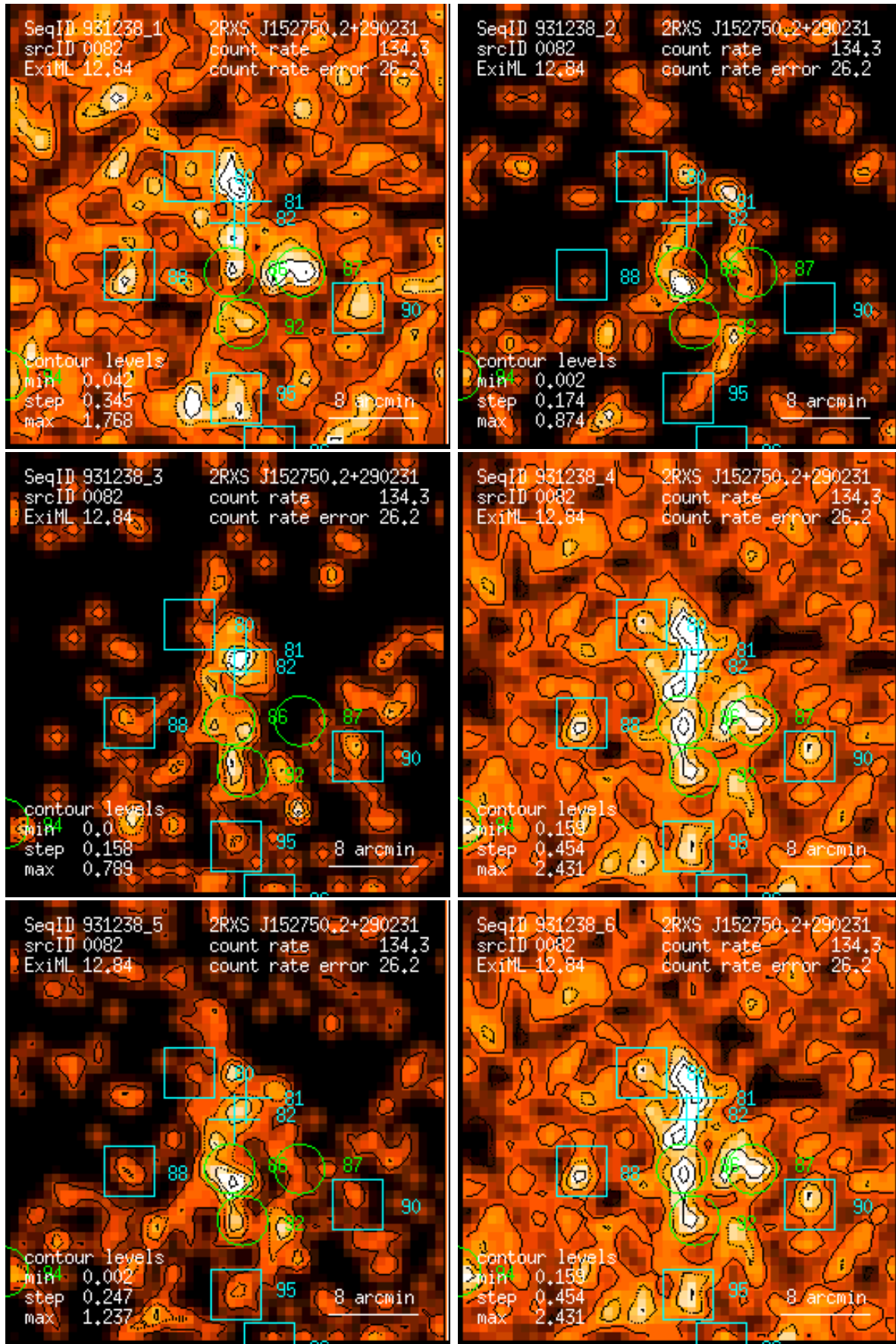
Figure 82: RASS 931238: detection 0082: band rate images, Gaussian filter: (1) PSPC channels 11 – 41, (2) 52 – 90, (3) 91 – 201, (4) 11 – 235, (5) 52 – 201, (6) 11 – 201. Broad band rates in counts/ks. Band rate contour levels in counts/ks/arcmin 2 .
