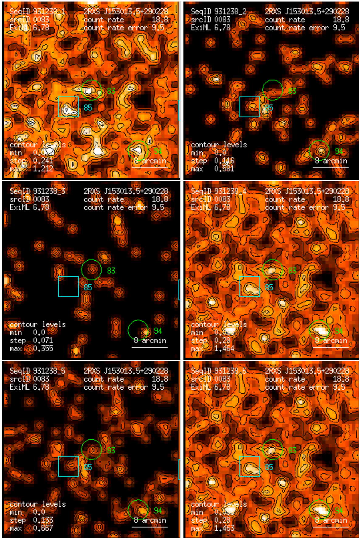
Figure 83: RASS 931238: detection 0083: band rate images, Gaussian filter: (1) PSPC channels 11 – 41, (2) 52 – 90, (3) 91 – 201, (4) 11 – 235, (5) 52 – 201, (6) 11 – 201. Broad band rates in counts/ks. Band rate contour levels in counts/ks/arcmin 2 .
