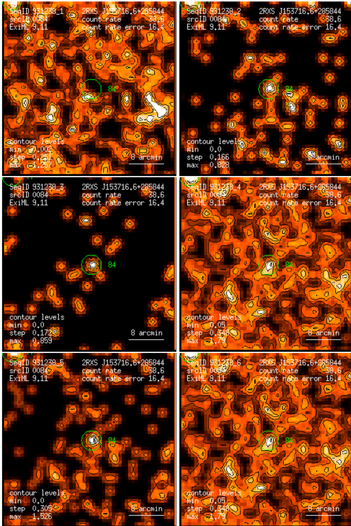
Figure 84: RASS 931238: detection 0084: band rate images, Gaussian filter: (1) PSPC channels 11 – 41, (2) 52 – 90, (3) 91 – 201, (4) 11 – 235, (5) 52 – 201, (6) 11 – 201. Broad band rates in counts/ks. Band rate contour levels in counts/ks/arcmin 2 .
