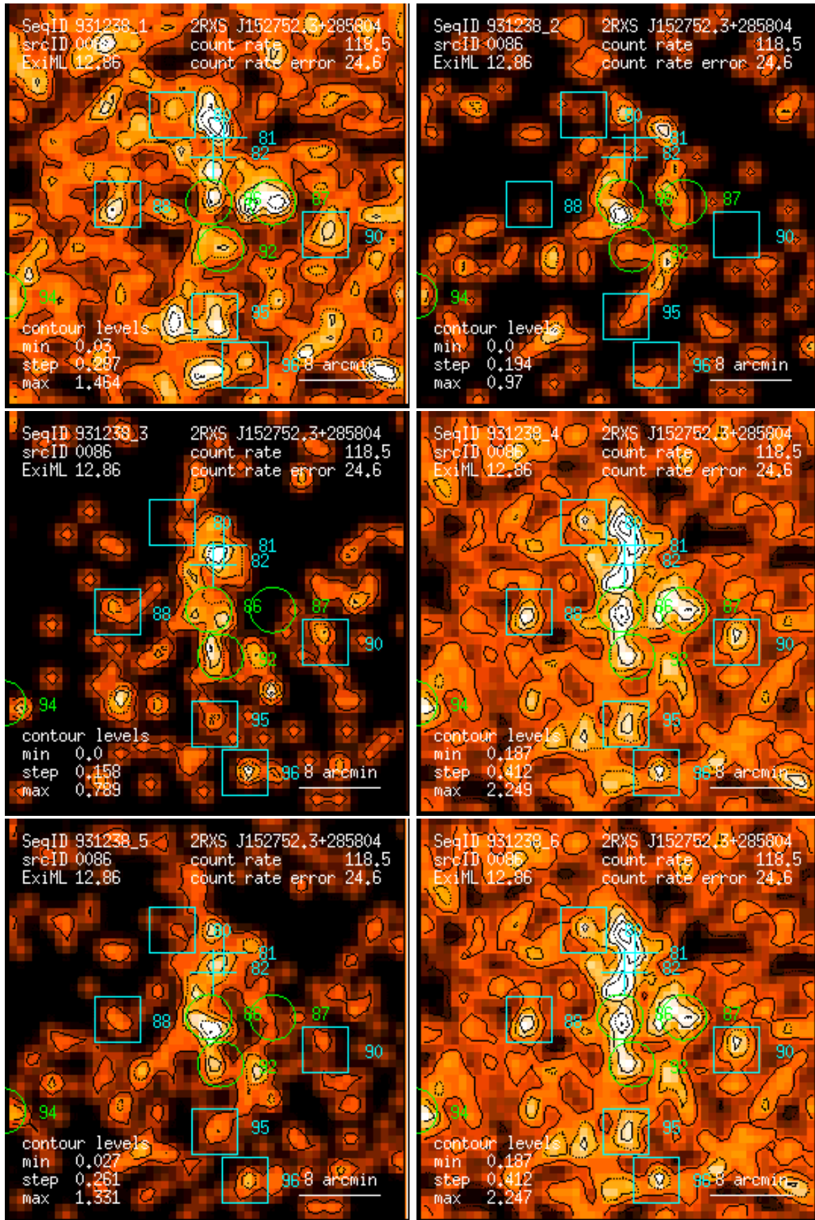
Figure 86: RASS 931238: detection 0086: band rate images, Gaussian filter: (1) PSPC channels 11 – 41, (2) 52 – 90, (3) 91 – 201, (4) 11 – 235, (5) 52 – 201, (6) 11 – 201. Broad band rates in counts/ks. Band rate contour levels in counts/ks/arcmin 2 .
