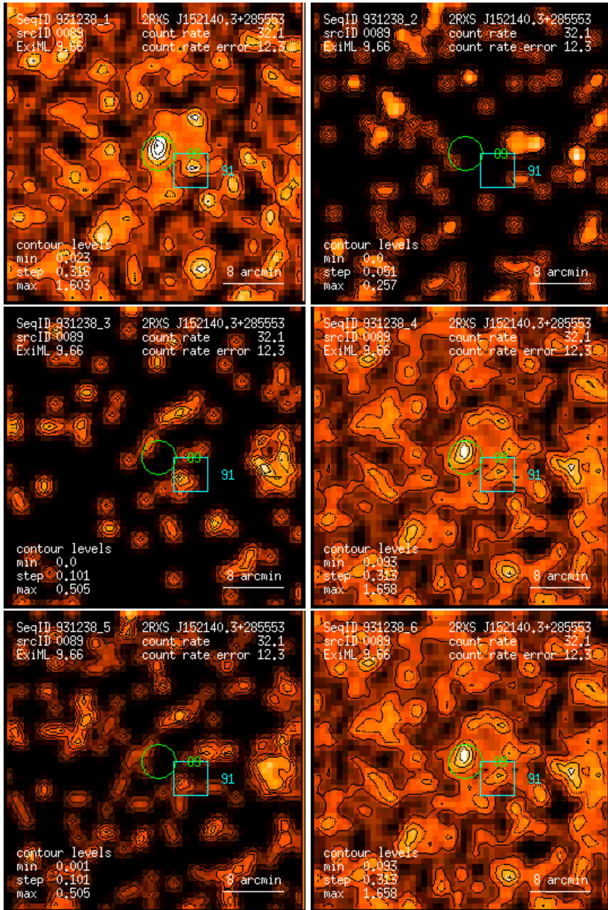
Figure 89: RASS 931238: detection 0089: band rate images, Gaussian filter: (1) PSPC channels 11 – 41, (2) 52 – 90, (3) 91 – 201, (4) 11 – 235, (5) 52 – 201, (6) 11 – 201. Broad band rates in counts/ks. Band rate contour levels in counts/ks/arcmin 2 .
