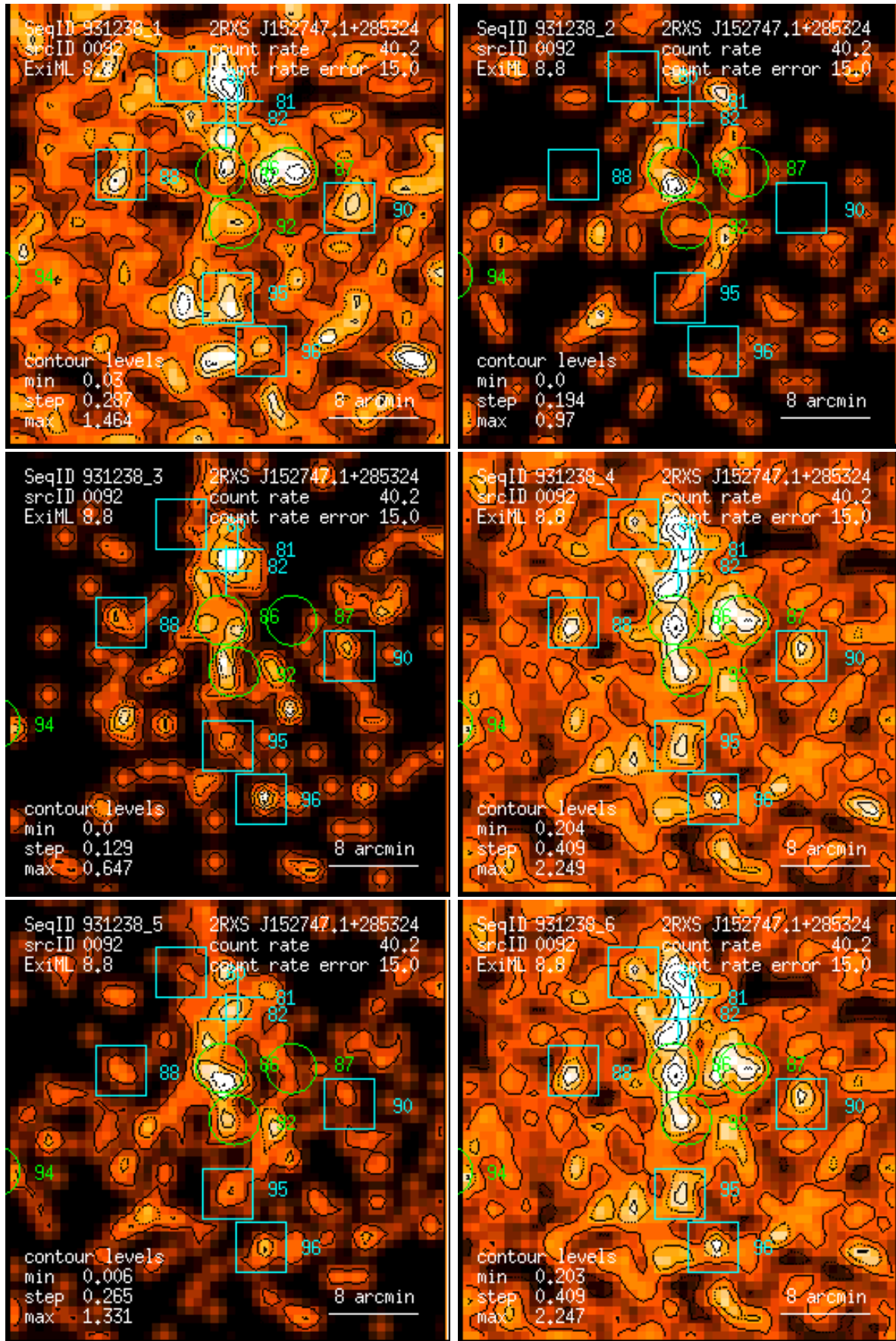
Figure 92: RASS 931238: detection 0092: band rate images, Gaussian filter: (1) PSPC channels 11 – 41, (2) 52 – 90, (3) 91 – 201, (4) 11 – 235, (5) 52 – 201, (6) 11 – 201. Broad band rates in counts/ks. Band rate contour levels in counts/ks/arcmin 2 .
