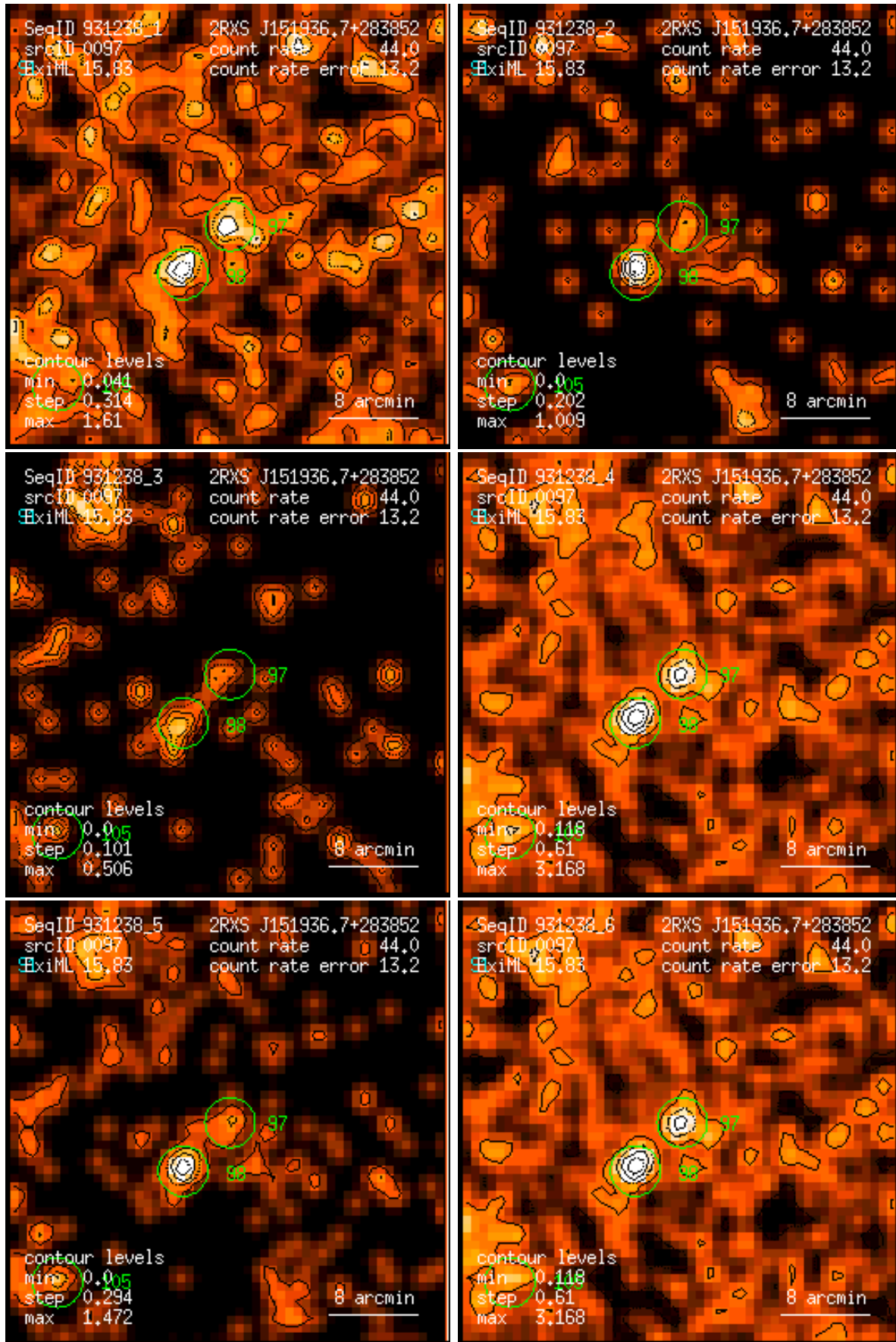
Figure 97: RASS 931238: detection 0097: band rate images, Gaussian filter: (1) PSPC channels 11 – 41, (2) 52 – 90, (3) 91 – 201, (4) 11 – 235, (5) 52 – 201, (6) 11 – 201. Broad band rates in counts/ks. Band rate contour levels in counts/ks/arcmin 2 .
