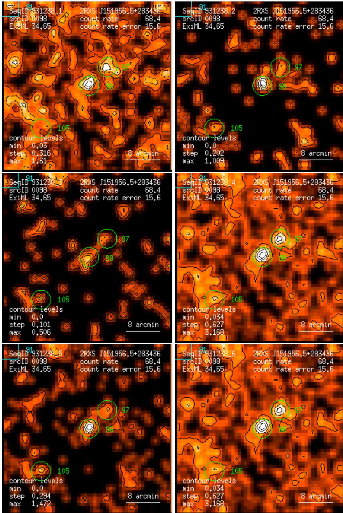
Figure 98: RASS 931238: detection 0098: band rate images, Gaussian filter: (1) PSPC channels 11 – 41, (2) 52 – 90, (3) 91 – 201, (4) 11 – 235, (5) 52 – 201, (6) 11 – 201. Broad band rates in counts/ks. Band rate contour levels in counts/ks/arcmin 2 .
