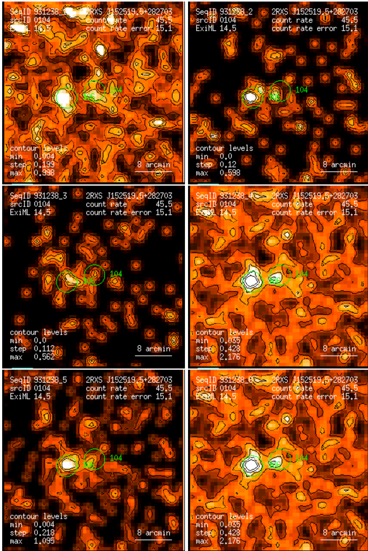
Figure 104: RASS 931238: detection 0104: band rate images, Gaussian filter: (1) PSPC channels 11 – 41, (2) 52 – 90, (3) 91 – 201, (4) 11 – 235, (5) 52 – 201, (6) 11 – 201. Broad band rates in counts/ks. Band rate contour levels in counts/ks/arcmin 2 .
