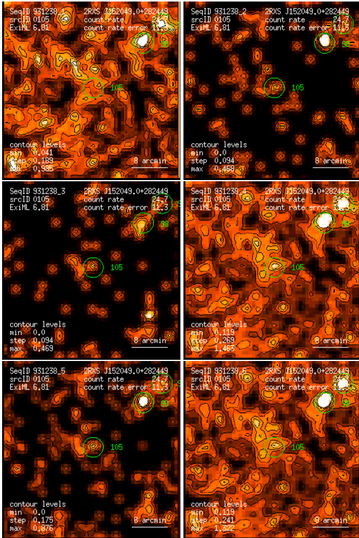
Figure 105: RASS 931238: detection 0105: band rate images, Gaussian filter: (1) PSPC channels 11 – 41, (2) 52 – 90, (3) 91 – 201, (4) 11 – 235, (5) 52 – 201, (6) 11 – 201. Broad band rates in counts/ks. Band rate contour levels in counts/ks/arcmin 2 .
