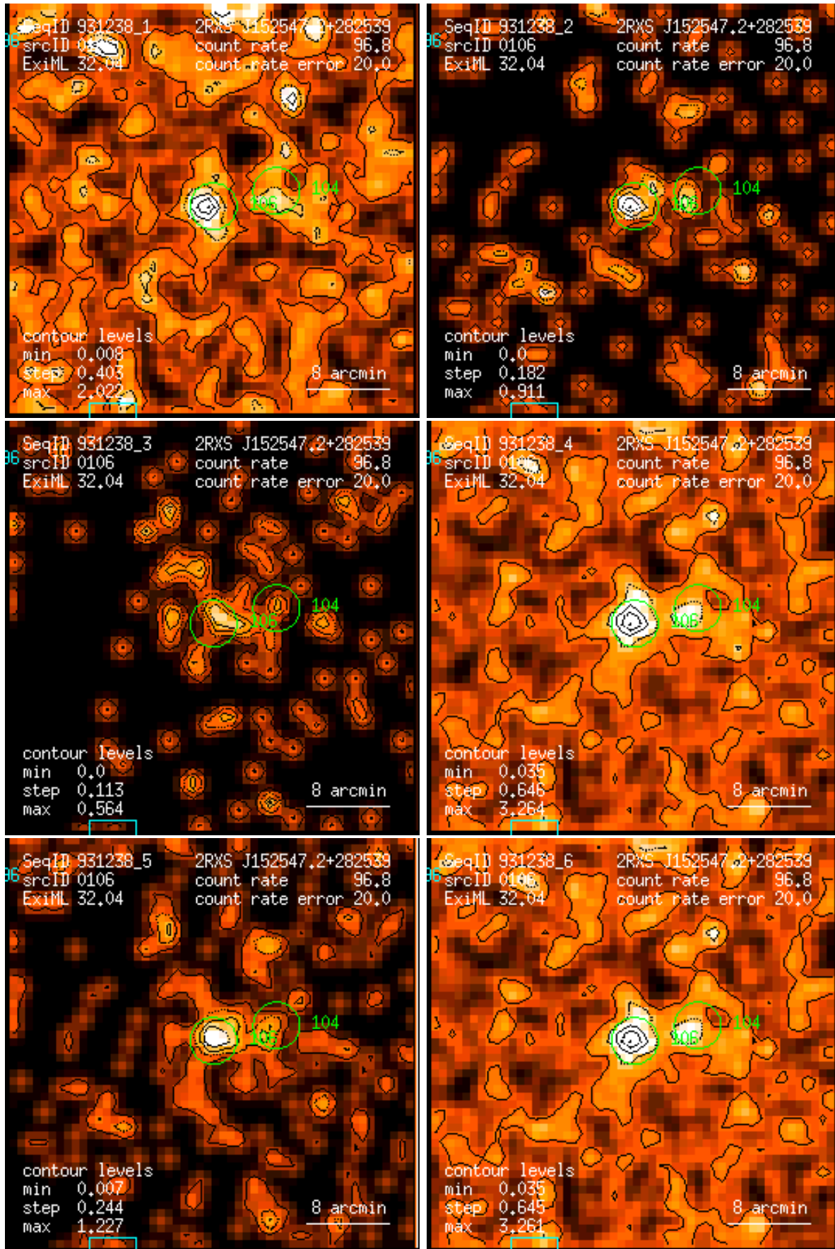
Figure 106: RASS 931238: detection 0106: band rate images, Gaussian filter: (1) PSPC channels 11 – 41, (2) 52 – 90, (3) 91 – 201, (4) 11 – 235, (5) 52 – 201, (6) 11 – 201. Broad band rates in counts/ks. Band rate contour levels in counts/ks/arcmin 2 .
