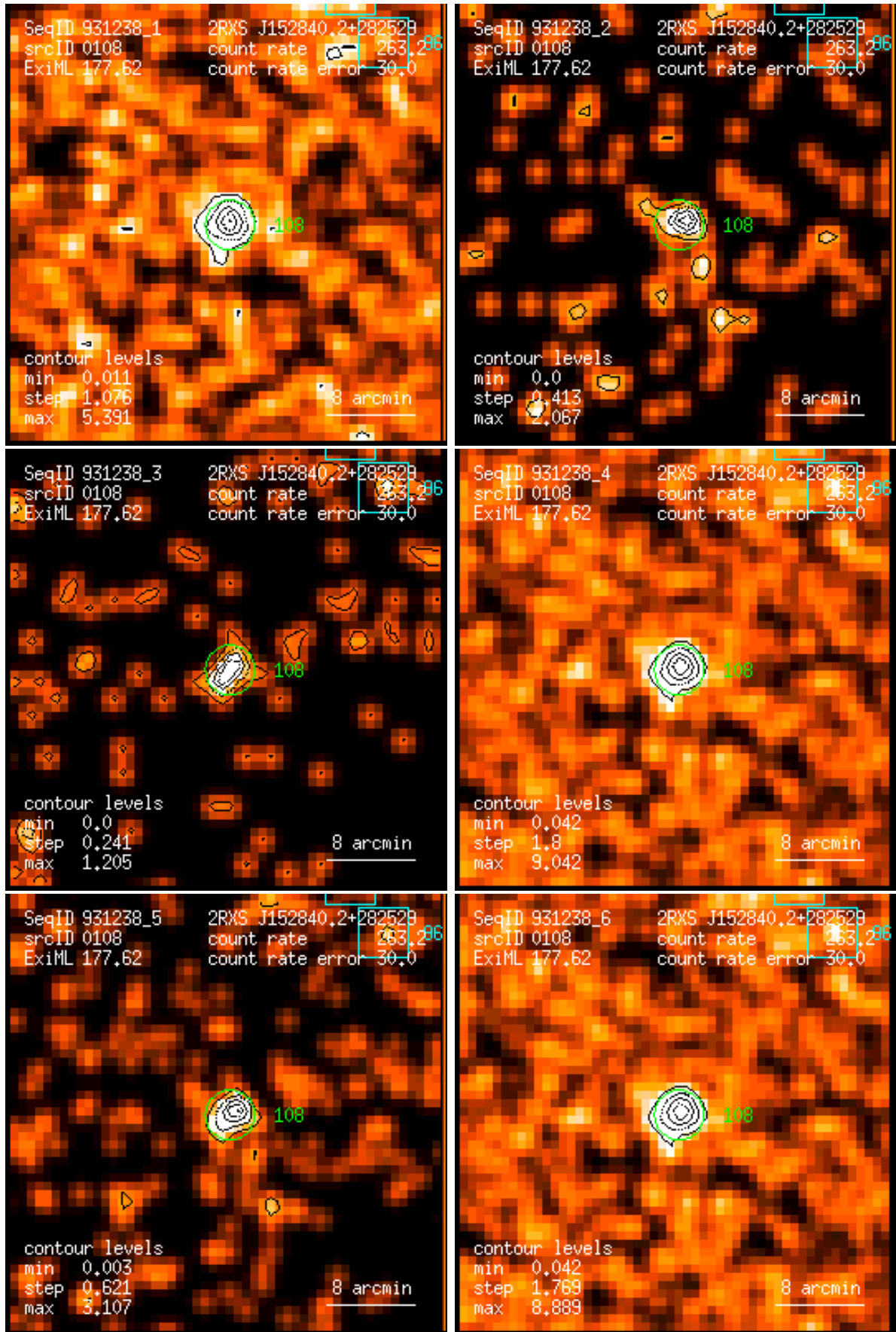
Figure 108: RASS 931238: detection 0108: band rate images, Gaussian filter: (1) PSPC channels 11 – 41, (2) 52 – 90, (3) 91 – 201, (4) 11 – 235, (5) 52 – 201, (6) 11 – 201. Broad band rates in counts/ks. Band rate contour levels in counts/ks/arcmin 2 .
