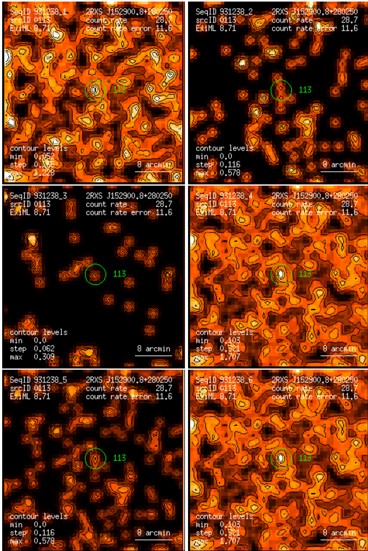
Figure 113: RASS 931238: detection 0113: band rate images, Gaussian filter: (1) PSPC channels 11 – 41, (2) 52 – 90, (3) 91 – 201, (4) 11 – 235, (5) 52 – 201, (6) 11 – 201. Broad band rates in counts/ks. Band rate contour levels in counts/ks/arcmin 2 .
