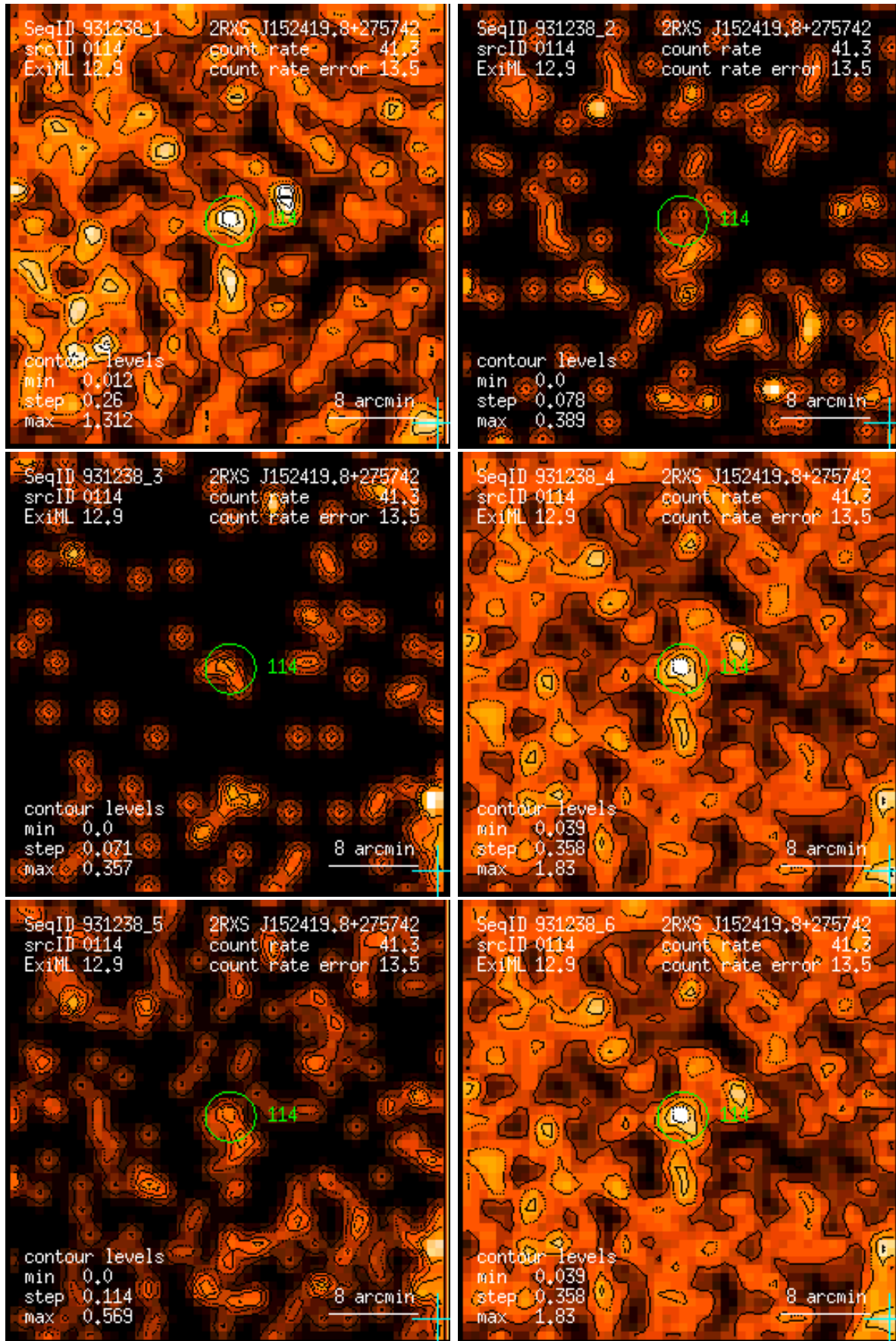
Figure 114: RASS 931238: detection 0114: band rate images, Gaussian filter: (1) PSPC channels 11 – 41, (2) 52 – 90, (3) 91 – 201, (4) 11 – 235, (5) 52 – 201, (6) 11 – 201. Broad band rates in counts/ks. Band rate contour levels in counts/ks/arcmin 2 .
