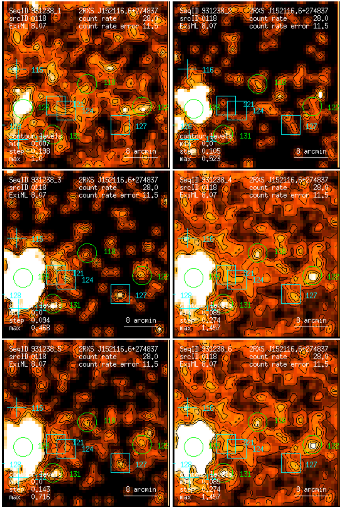
Figure 118: RASS 931238: detection 0118: band rate images, Gaussian filter: (1) PSPC channels 11 – 41, (2) 52 – 90, (3) 91 – 201, (4) 11 – 235, (5) 52 – 201, (6) 11 – 201. Broad band rates in counts/ks. Band rate contour levels in counts/ks/arcmin 2 .
