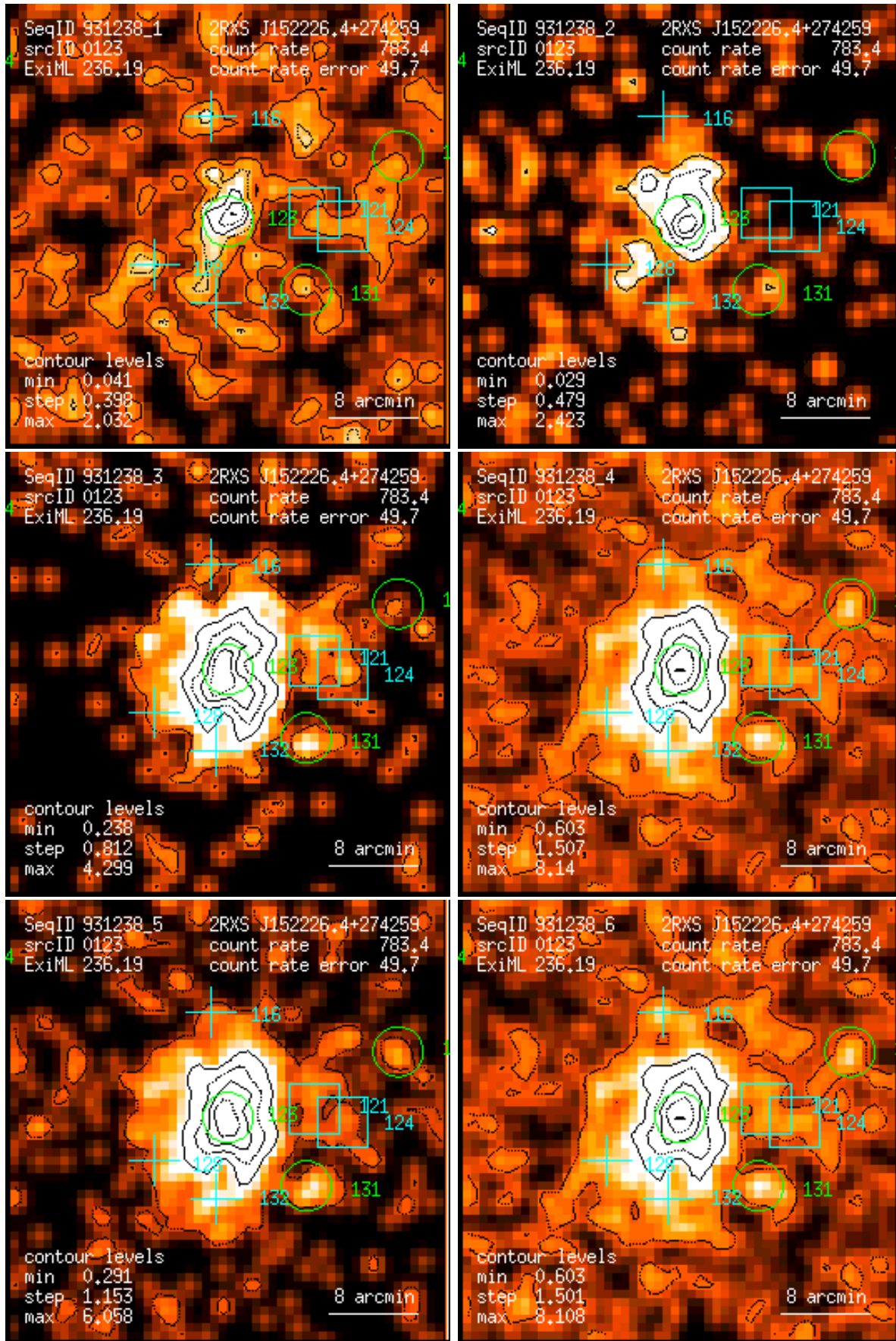
Figure 123: RASS 931238: detection 0123: band rate images, Gaussian filter: (1) PSPC channels 11 – 41, (2) 52 – 90, (3) 91 – 201, (4) 11 – 235, (5) 52 – 201, (6) 11 – 201. Broad band rates in counts/ks. Band rate contour levels in counts/ks/arcmin 2 .
