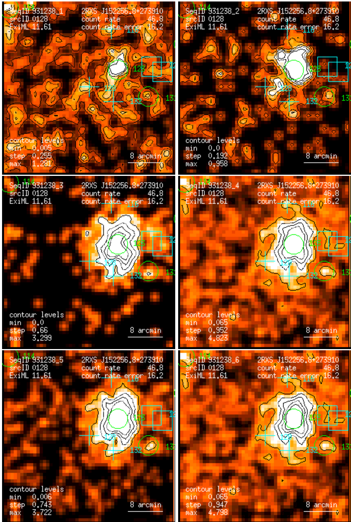
Figure 128: RASS 931238: detection 0128: band rate images, Gaussian filter: (1) PSPC channels 11 – 41, (2) 52 – 90, (3) 91 – 201, (4) 11 – 235, (5) 52 – 201, (6) 11 – 201. Broad band rates in counts/ks. Band rate contour levels in counts/ks/arcmin 2 .
