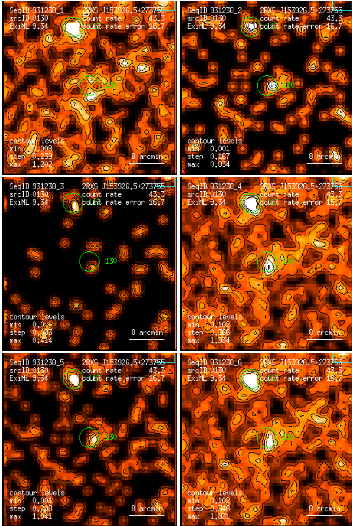
Figure 130: RASS 931238: detection 0130: band rate images, Gaussian filter: (1) PSPC channels 11 – 41, (2) 52 – 90, (3) 91 – 201, (4) 11 – 235, (5) 52 – 201, (6) 11 – 201. Broad band rates in counts/ks. Band rate contour levels in counts/ks/arcmin 2 .
