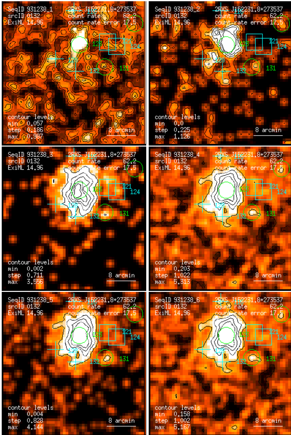
Figure 132: RASS 931238: detection 0132: band rate images, Gaussian filter: (1) PSPC channels 11 – 41, (2) 52 – 90, (3) 91 – 201, (4) 11 – 235, (5) 52 – 201, (6) 11 – 201. Broad band rates in counts/ks. Band rate contour levels in counts/ks/arcmin 2 .
