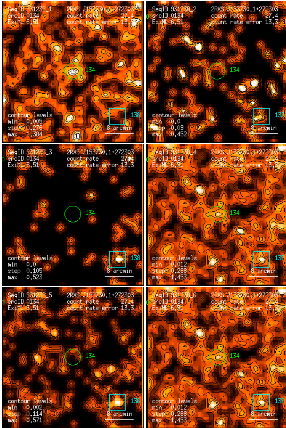
Figure 134: RASS 931238: detection 0134: band rate images, Gaussian filter: (1) PSPC channels 11 – 41, (2) 52 – 90, (3) 91 – 201, (4) 11 – 235, (5) 52 – 201, (6) 11 – 201. Broad band rates in counts/ks. Band rate contour levels in counts/ks/arcmin 2 .
