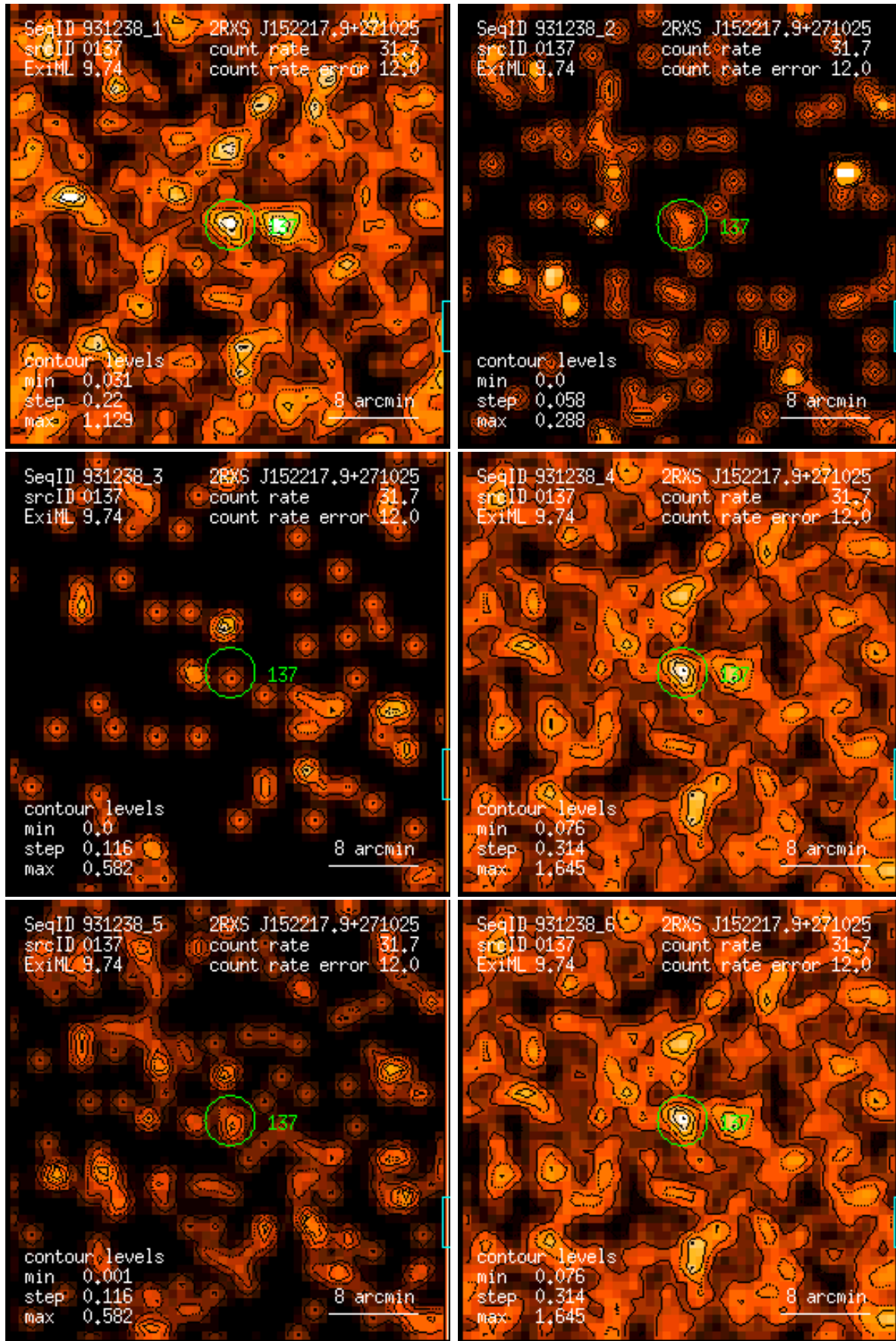
Figure 137: RASS 931238: detection 0137: band rate images, Gaussian filter: (1) PSPC channels 11 – 41, (2) 52 – 90, (3) 91 – 201, (4) 11 – 235, (5) 52 – 201, (6) 11 – 201. Broad band rates in counts/ks. Band rate contour levels in counts/ks/arcmin 2 .
