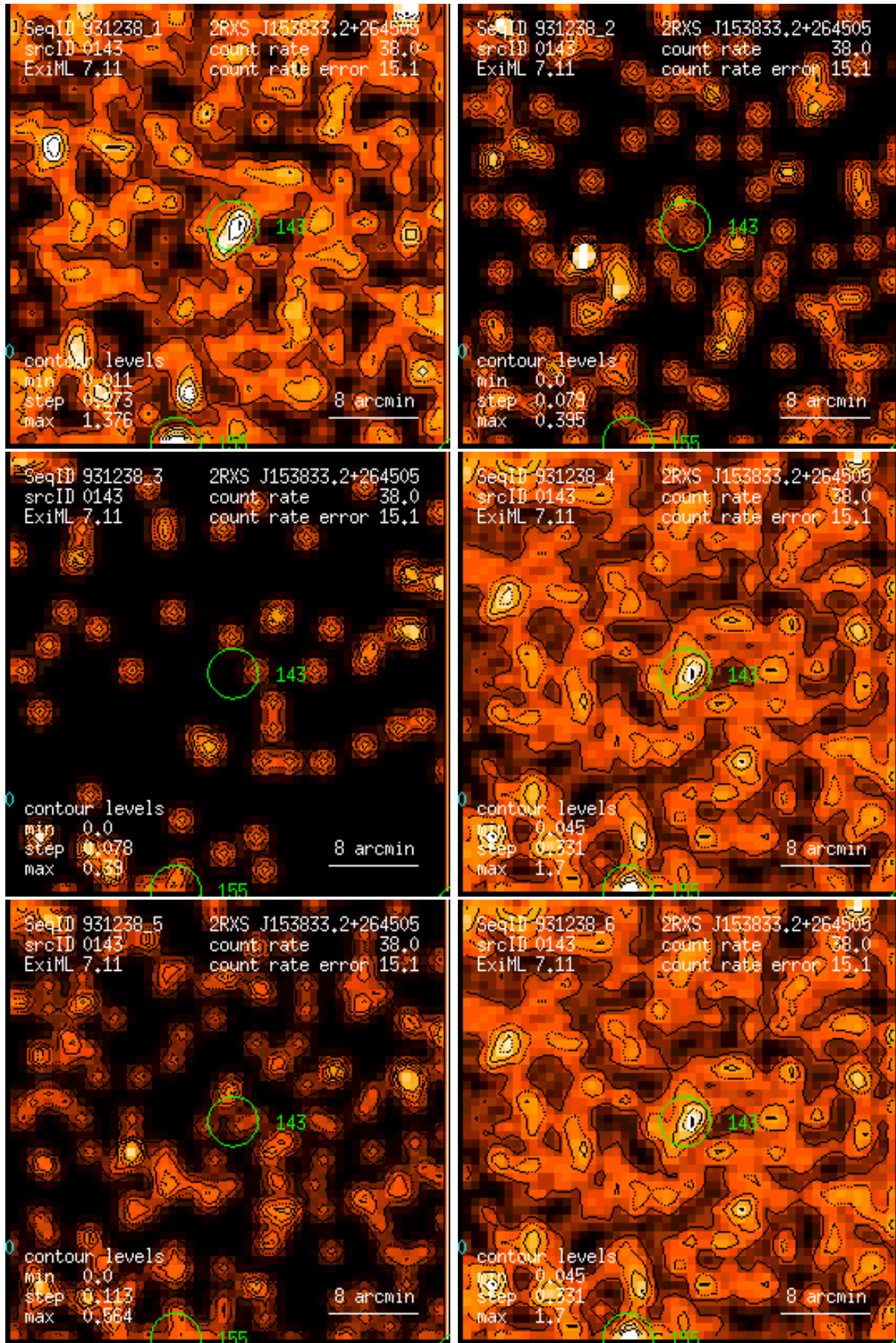
Figure 143: RASS 931238: detection 0143: band rate images, Gaussian filter: (1) PSPC channels 11 – 41, (2) 52 – 90, (3) 91 – 201, (4) 11 – 235, (5) 52 – 201, (6) 11 – 201. Broad band rates in counts/ks. Band rate contour levels in counts/ks/arcmin 2 .
