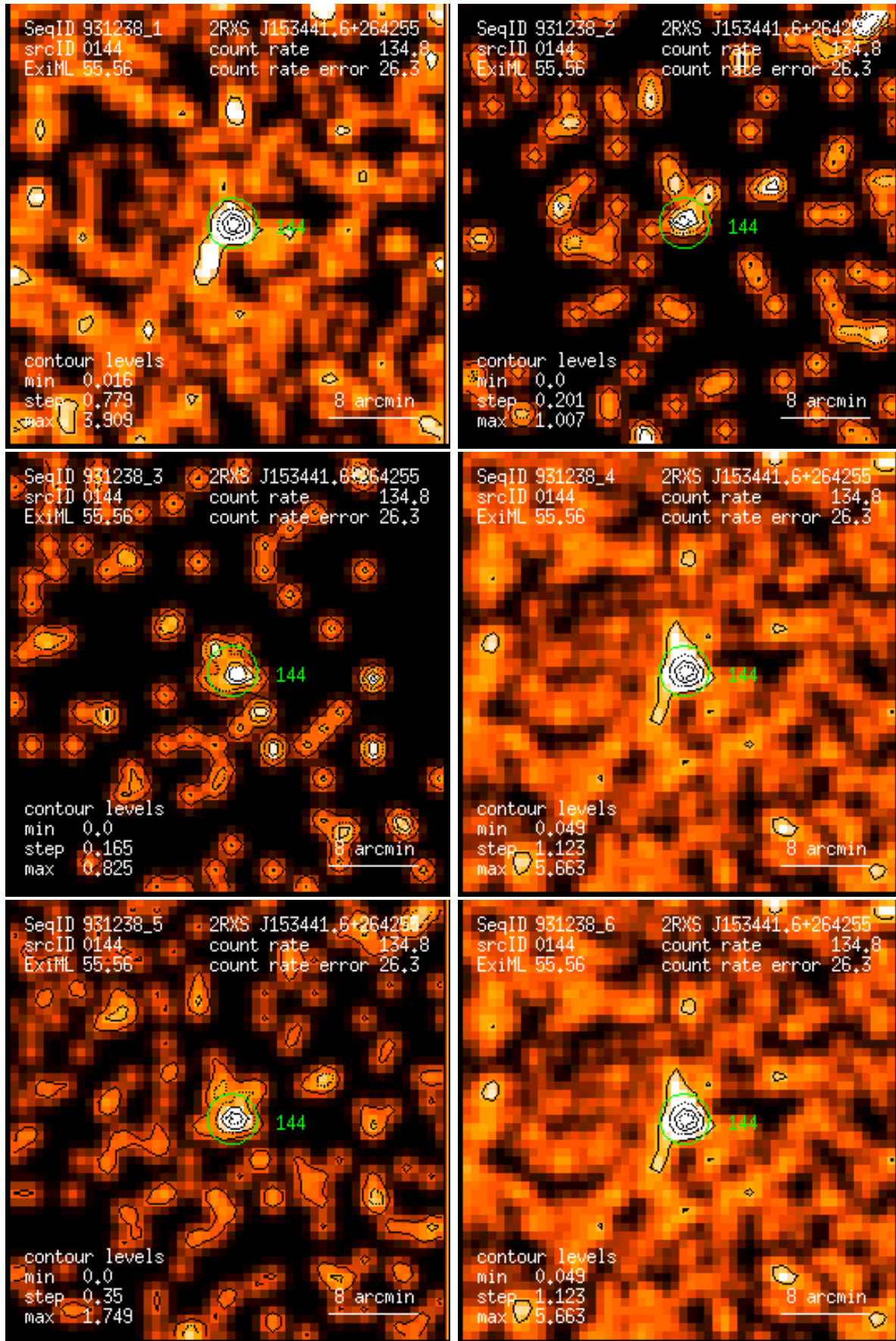
Figure 144: RASS 931238: detection 0144: band rate images, Gaussian filter: (1) PSPC channels 11 – 41, (2) 52 – 90, (3) 91 – 201, (4) 11 – 235, (5) 52 – 201, (6) 11 – 201. Broad band rates in counts/ks. Band rate contour levels in counts/ks/arcmin 2 .
