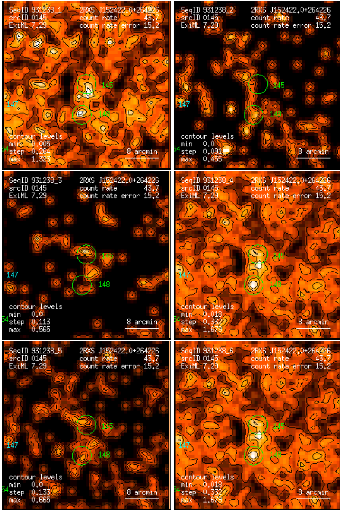
Figure 145: RASS 931238: detection 0145: band rate images, Gaussian filter: (1) PSPC channels 11 – 41, (2) 52 – 90, (3) 91 – 201, (4) 11 – 235, (5) 52 – 201, (6) 11 – 201. Broad band rates in counts/ks. Band rate contour levels in counts/ks/arcmin 2 .
