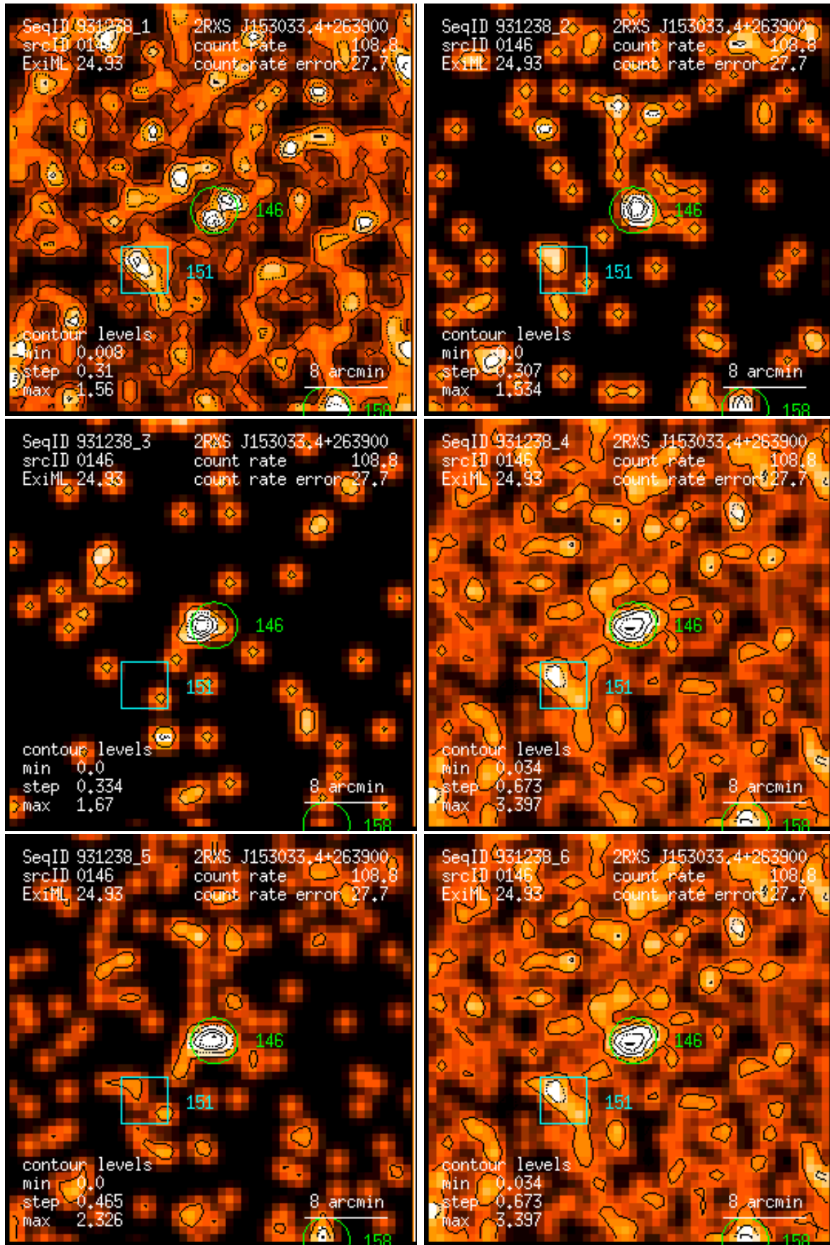
Figure 146: RASS 931238: detection 0146: band rate images, Gaussian filter: (1) PSPC channels 11 – 41, (2) 52 – 90, (3) 91 – 201, (4) 11 – 235, (5) 52 – 201, (6) 11 – 201. Broad band rates in counts/ks. Band rate contour levels in counts/ks/arcmin 2 .
