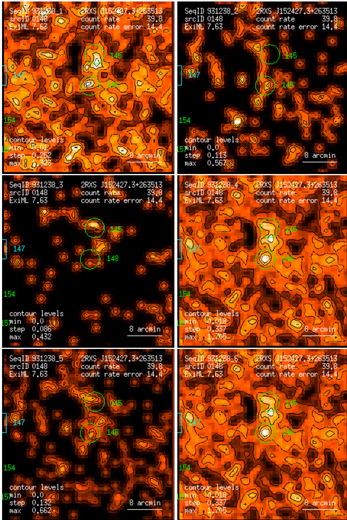
Figure 148: RASS 931238: detection 0148: band rate images, Gaussian filter: (1) PSPC channels 11 – 41, (2) 52 – 90, (3) 91 – 201, (4) 11 – 235, (5) 52 – 201, (6) 11 – 201. Broad band rates in counts/ks. Band rate contour levels in counts/ks/arcmin 2 .
