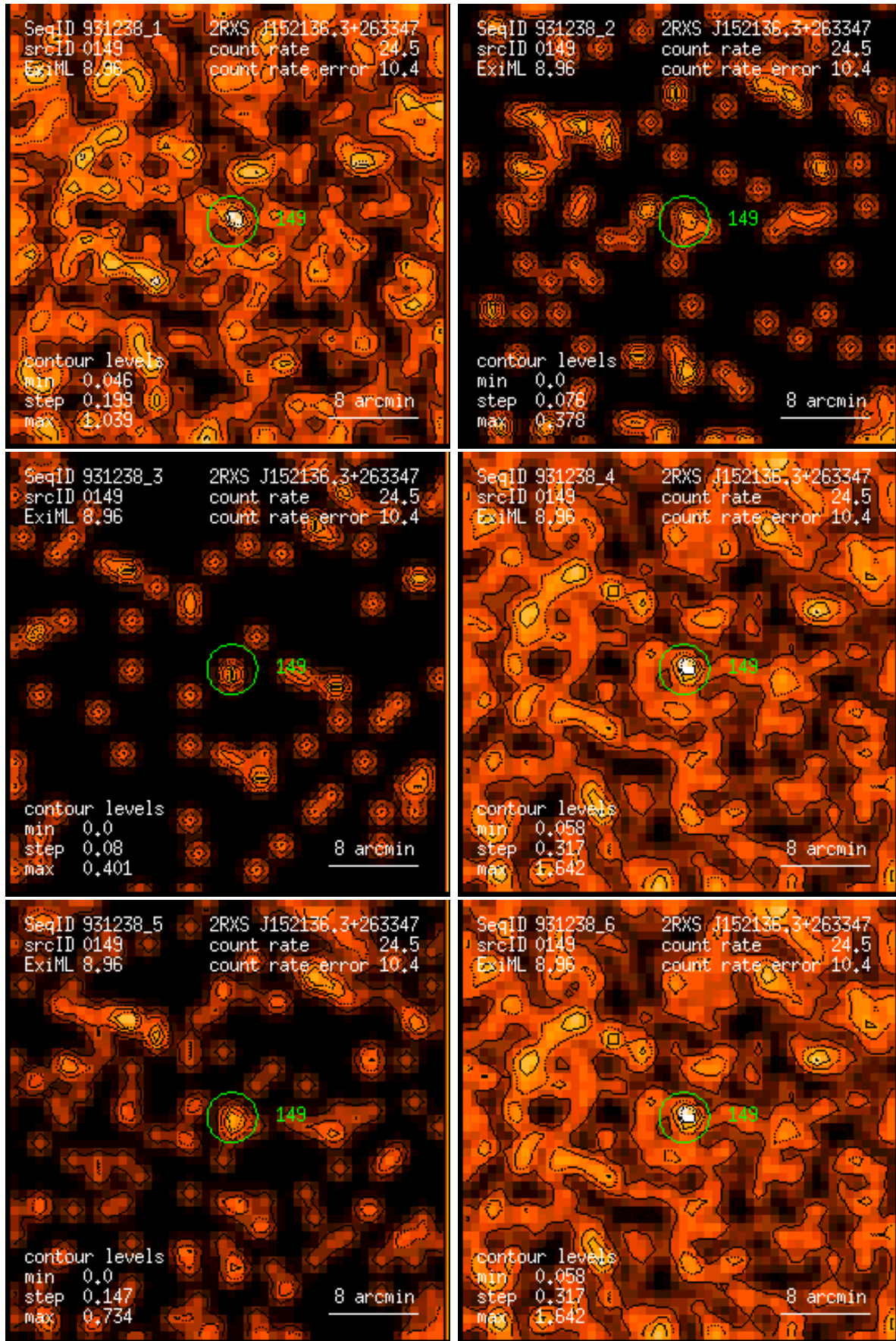
Figure 149: RASS 931238: detection 0149: band rate images, Gaussian filter: (1) PSPC channels 11 – 41, (2) 52 – 90, (3) 91 – 201, (4) 11 – 235, (5) 52 – 201, (6) 11 – 201. Broad band rates in counts/ks. Band rate contour levels in counts/ks/arcmin 2 .
