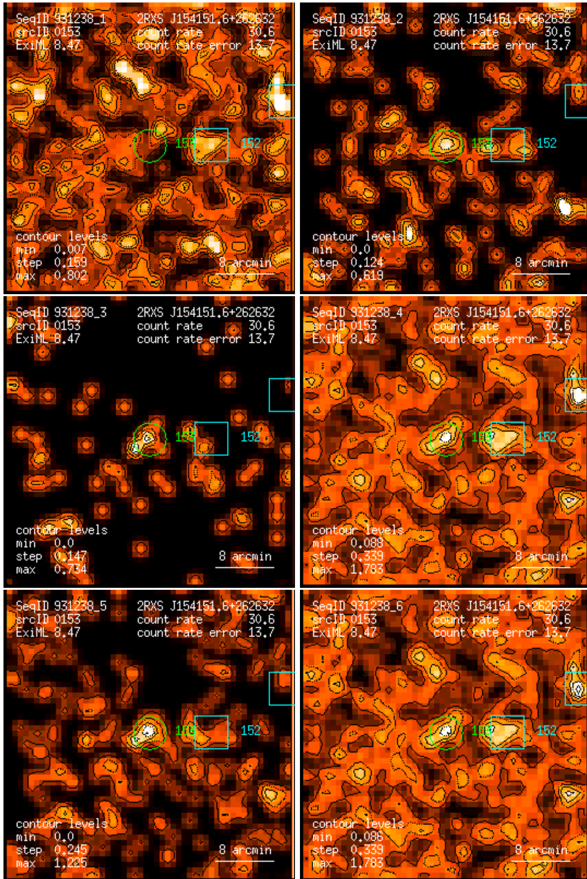
Figure 153: RASS 931238: detection 0153: band rate images, Gaussian filter: (1) PSPC channels 11 – 41, (2) 52 – 90, (3) 91 – 201, (4) 11 – 235, (5) 52 – 201, (6) 11 – 201. Broad band rates in counts/ks. Band rate contour levels in counts/ks/arcmin 2 .
