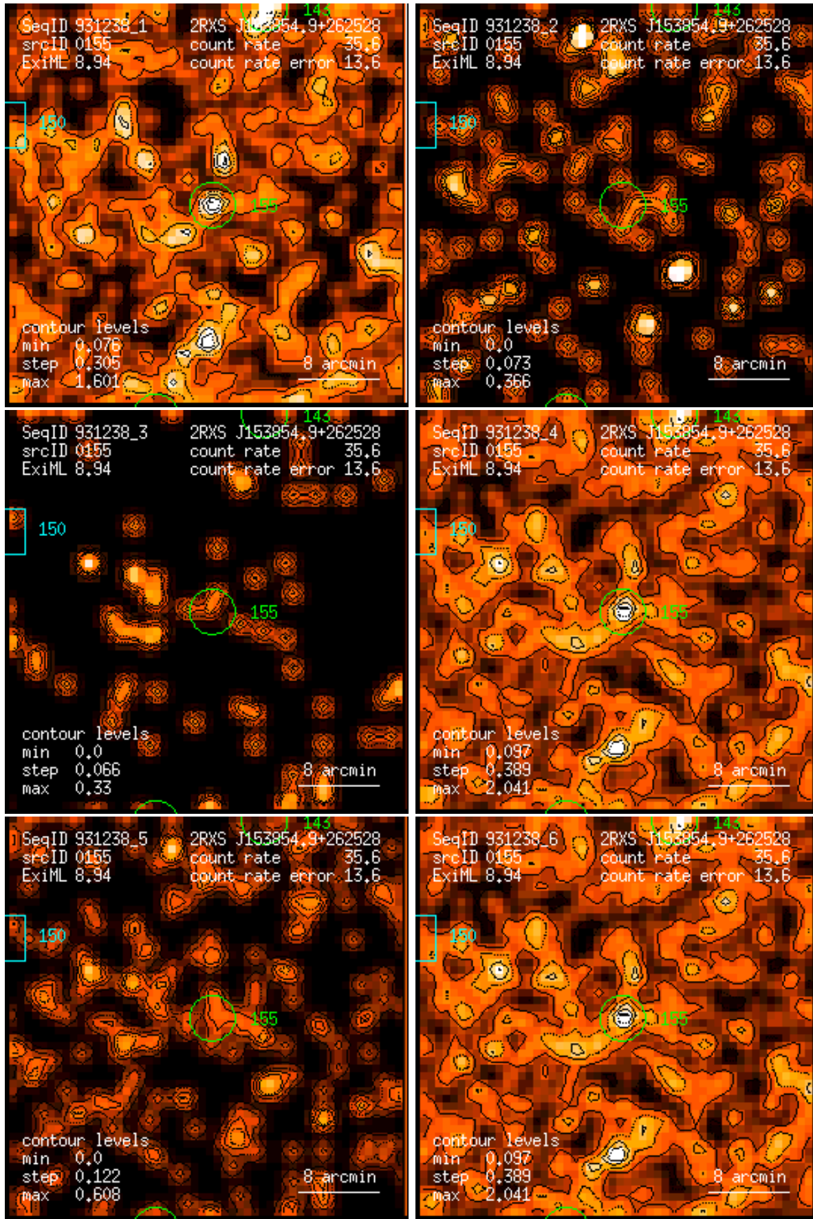
Figure 155: RASS 931238: detection 0155: band rate images, Gaussian filter: (1) PSPC channels 11 – 41, (2) 52 – 90, (3) 91 – 201, (4) 11 – 235, (5) 52 – 201, (6) 11 – 201. Broad band rates in counts/ks. Band rate contour levels in counts/ks/arcmin 2 .
