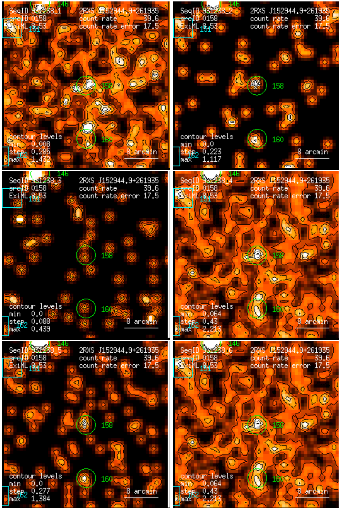
Figure 158: RASS 931238: detection 0158: band rate images, Gaussian filter: (1) PSPC channels 11 – 41, (2) 52 – 90, (3) 91 – 201, (4) 11 – 235, (5) 52 – 201, (6) 11 – 201. Broad band rates in counts/ks. Band rate contour levels in counts/ks/arcmin 2 .
