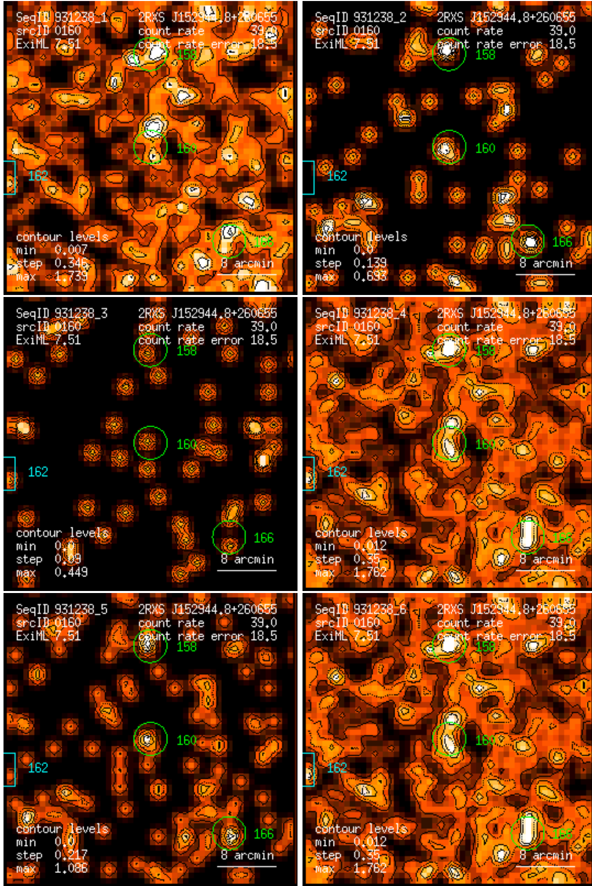
Figure 160: RASS 931238: detection 0160: band rate images, Gaussian filter: (1) PSPC channels 11 – 41, (2) 52 – 90, (3) 91 – 201, (4) 11 – 235, (5) 52 – 201, (6) 11 – 201. Broad band rates in counts/ks. Band rate contour levels in counts/ks/arcmin 2 .
