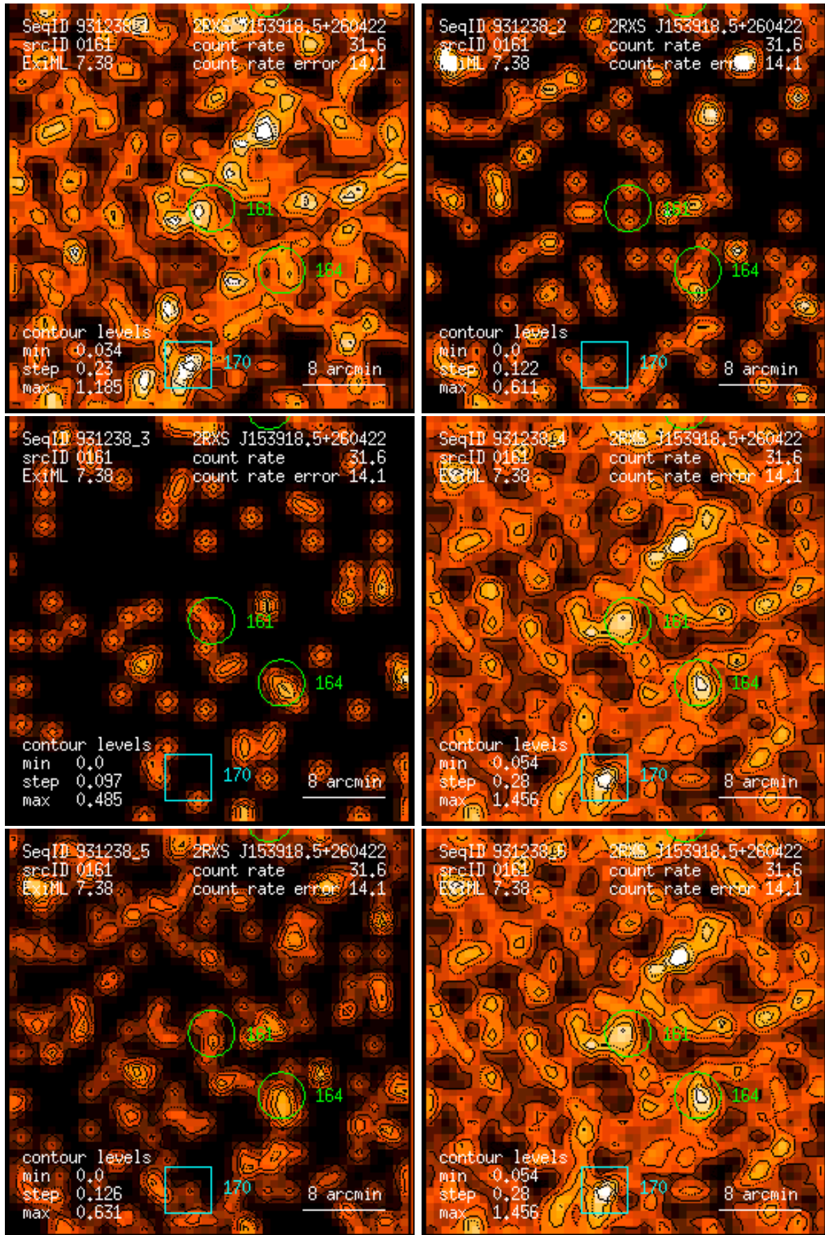
Figure 161: RASS 931238: detection 0161: band rate images, Gaussian filter: (1) PSPC channels 11 – 41, (2) 52 – 90, (3) 91 – 201, (4) 11 – 235, (5) 52 – 201, (6) 11 – 201. Broad band rates in counts/ks. Band rate contour levels in counts/ks/arcmin 2 .
