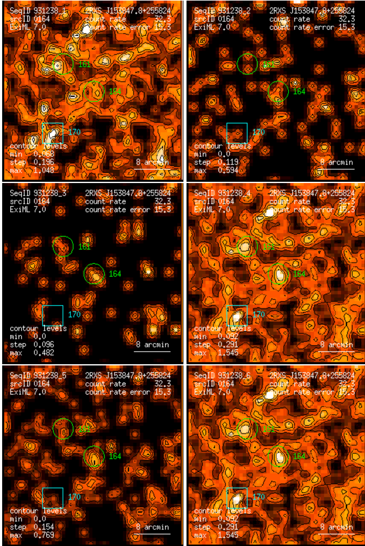
Figure 164: RASS 931238: detection 0164: band rate images, Gaussian filter: (1) PSPC channels 11 – 41, (2) 52 – 90, (3) 91 – 201, (4) 11 – 235, (5) 52 – 201, (6) 11 – 201. Broad band rates in counts/ks. Band rate contour levels in counts/ks/arcmin 2 .
