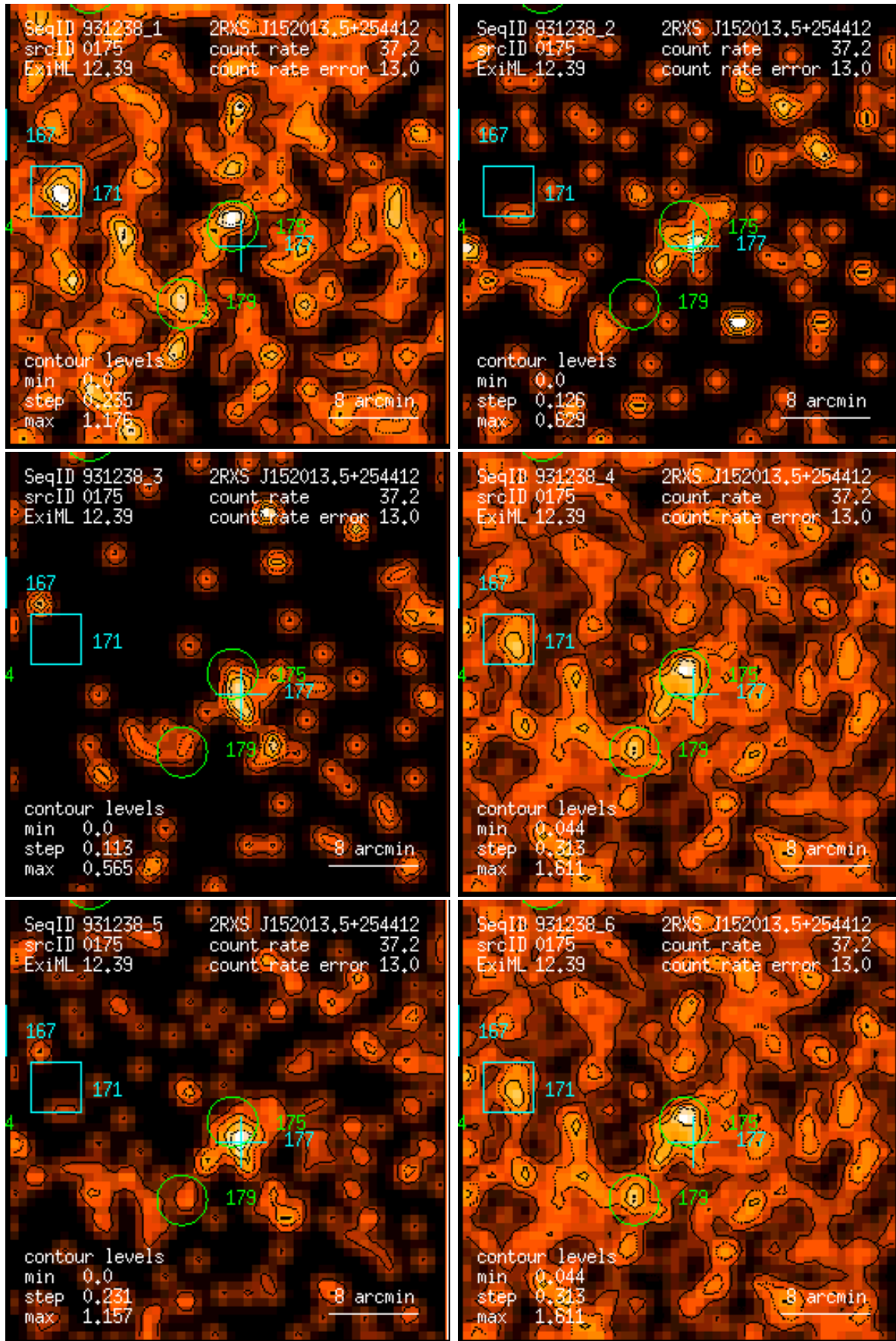
Figure 175: RASS 931238: detection 0175: band rate images, Gaussian filter: (1) PSPC channels 11 – 41, (2) 52 – 90, (3) 91 – 201, (4) 11 – 235, (5) 52 – 201, (6) 11 – 201. Broad band rates in counts/ks. Band rate contour levels in counts/ks/arcmin 2 .
