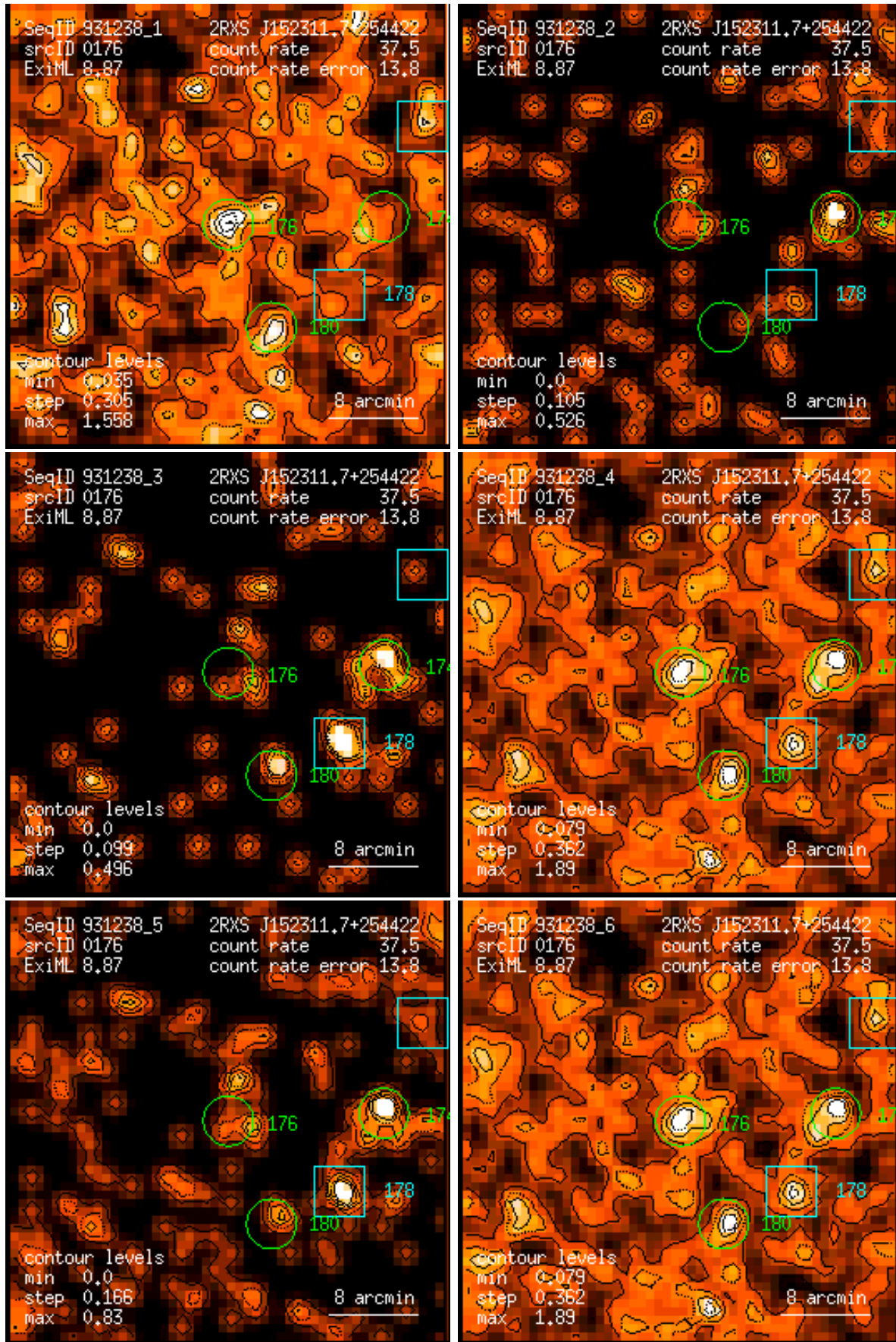
Figure 176: RASS 931238: detection 0176: band rate images, Gaussian filter: (1) PSPC channels 11 – 41, (2) 52 – 90, (3) 91 – 201, (4) 11 – 235, (5) 52 – 201, (6) 11 – 201. Broad band rates in counts/ks. Band rate contour levels in counts/ks/arcmin 2 .
