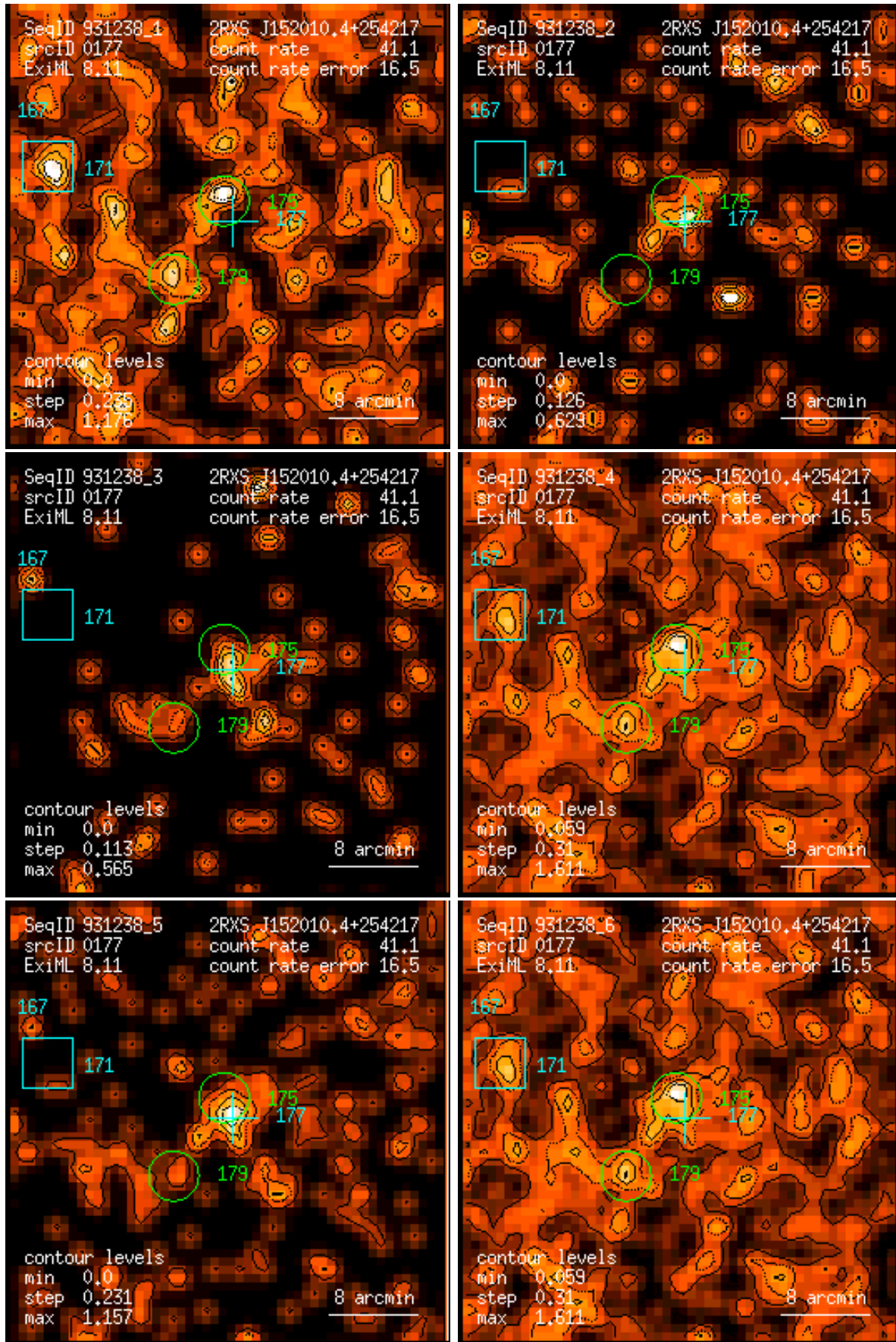
Figure 177: RASS 931238: detection 0177: band rate images, Gaussian filter: (1) PSPC channels 11 – 41, (2) 52 – 90, (3) 91 – 201, (4) 11 – 235, (5) 52 – 201, (6) 11 – 201. Broad band rates in counts/ks. Band rate contour levels in counts/ks/arcmin 2 .
