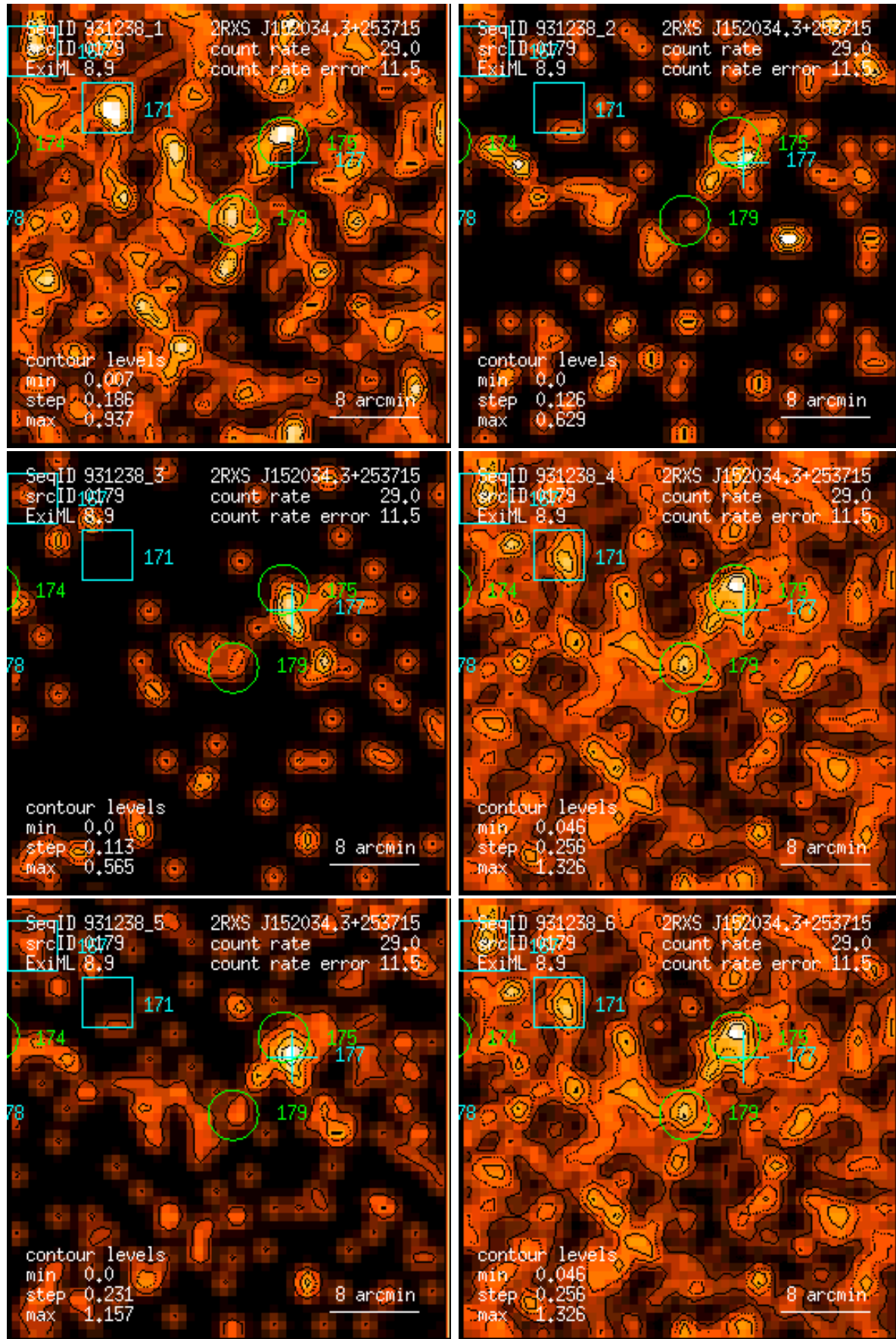
Figure 179: RASS 931238: detection 0179: band rate images, Gaussian filter: (1) PSPC channels 11 – 41, (2) 52 – 90, (3) 91 – 201, (4) 11 – 235, (5) 52 – 201, (6) 11 – 201. Broad band rates in counts/ks. Band rate contour levels in counts/ks/arcmin 2 .
