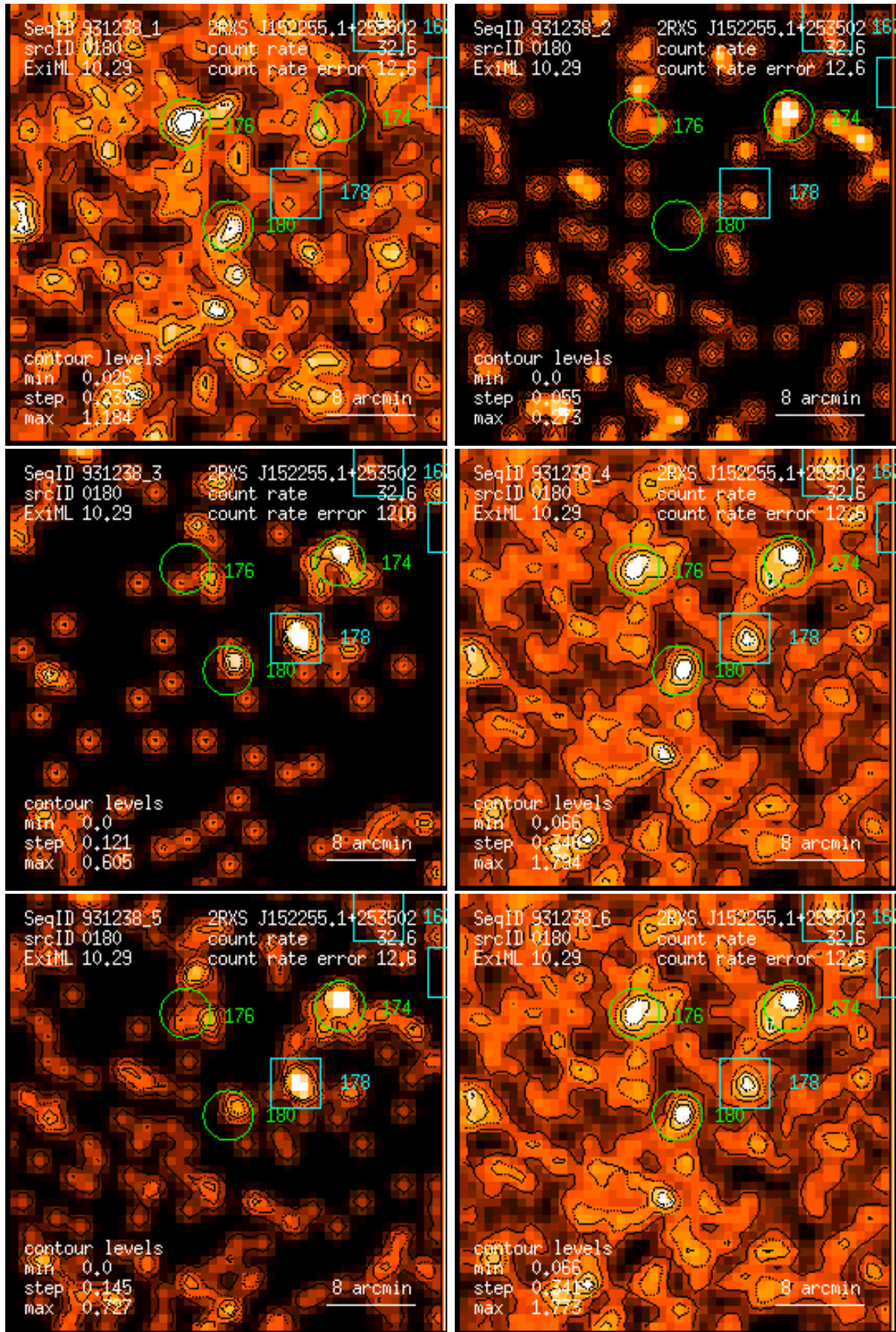
Figure 180: RASS 931238: detection 0180: band rate images, Gaussian filter: (1) PSPC channels 11 – 41, (2) 52 – 90, (3) 91 – 201, (4) 11 – 235, (5) 52 – 201, (6) 11 – 201. Broad band rates in counts/ks. Band rate contour levels in counts/ks/arcmin 2 .
