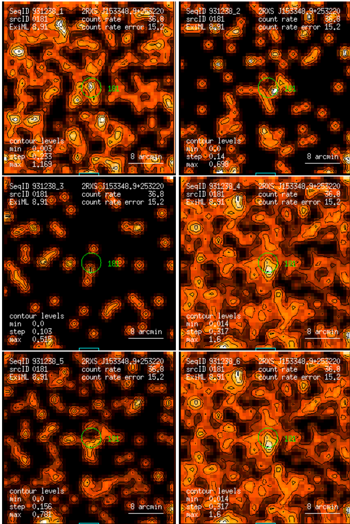
Figure 181: RASS 931238: detection 0181: band rate images, Gaussian filter: (1) PSPC channels 11 – 41, (2) 52 – 90, (3) 91 – 201, (4) 11 – 235, (5) 52 – 201, (6) 11 – 201. Broad band rates in counts/ks. Band rate contour levels in counts/ks/arcmin 2 .
