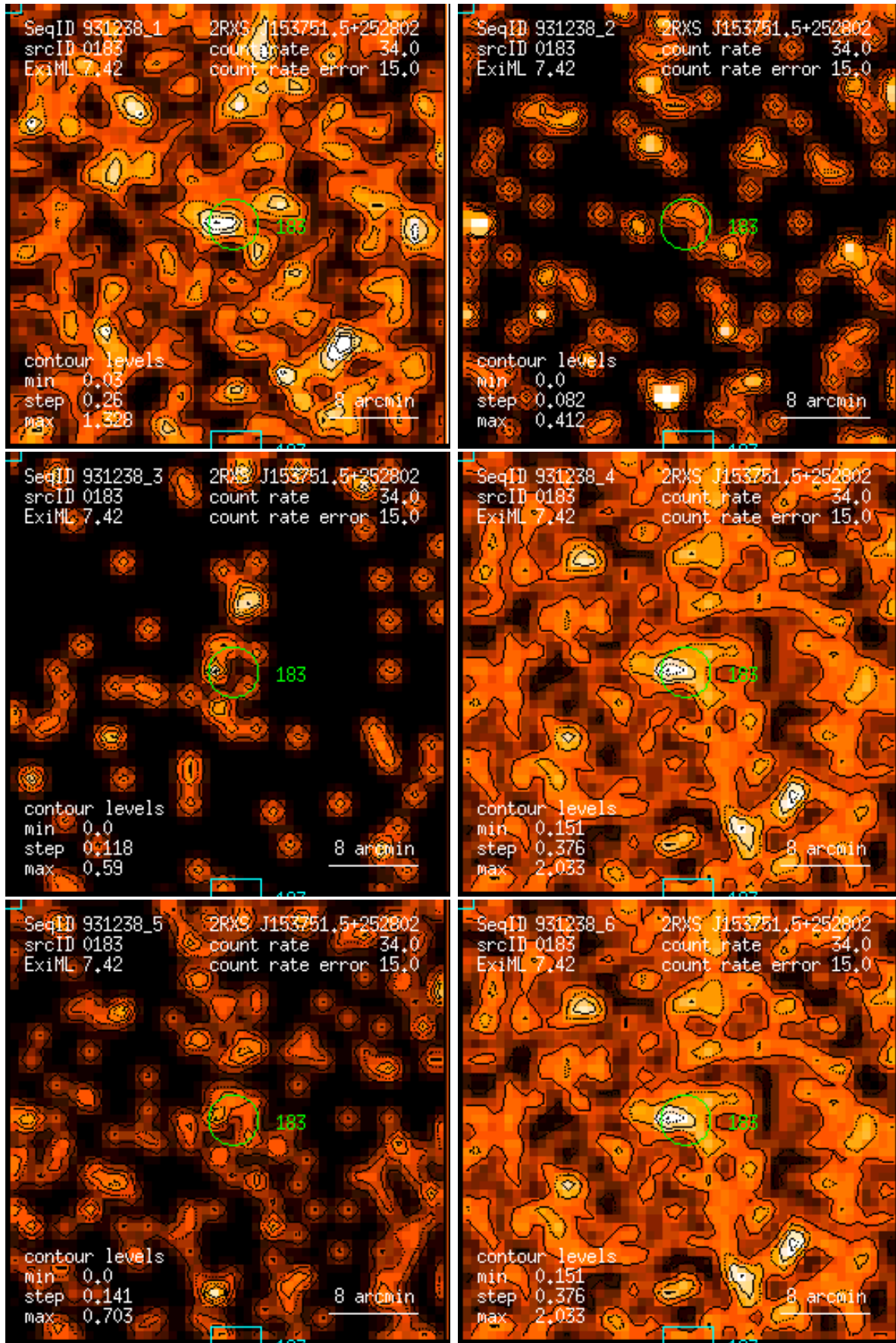
Figure 183: RASS 931238: detection 0183: band rate images, Gaussian filter: (1) PSPC channels 11 – 41, (2) 52 – 90, (3) 91 – 201, (4) 11 – 235, (5) 52 – 201, (6) 11 – 201. Broad band rates in counts/ks. Band rate contour levels in counts/ks/arcmin 2 .
