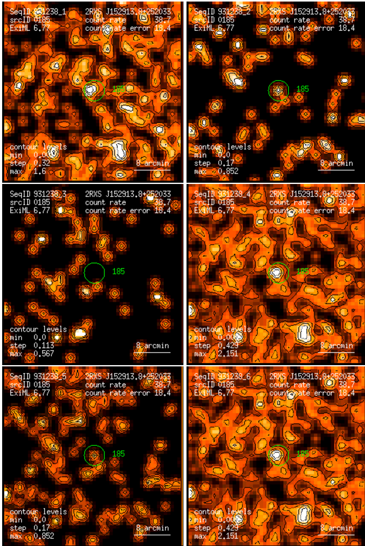
Figure 185: RASS 931238: detection 0185: band rate images, Gaussian filter: (1) PSPC channels 11 – 41, (2) 52 – 90, (3) 91 – 201, (4) 11 – 235, (5) 52 – 201, (6) 11 – 201. Broad band rates in counts/ks. Band rate contour levels in counts/ks/arcmin 2 .
